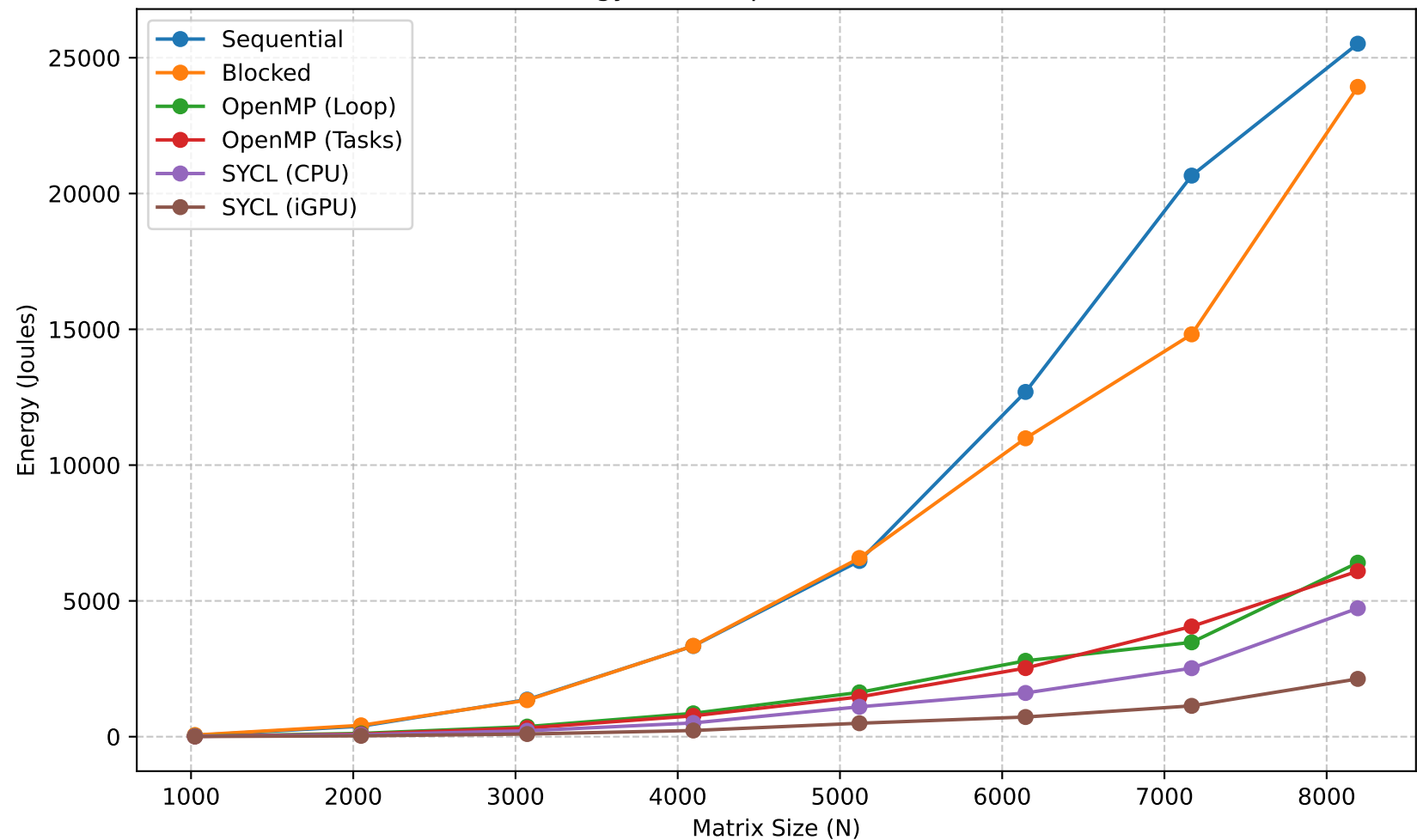
Energy Consumption vs Matrix Size
