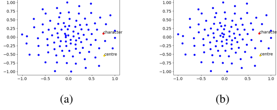
Figure 1: 2D plot of 100 embeddings from: (a) element-wise difference of original pretrained model, (b) element-wise difference of transformed model after 10 iterations of glide reflection.
