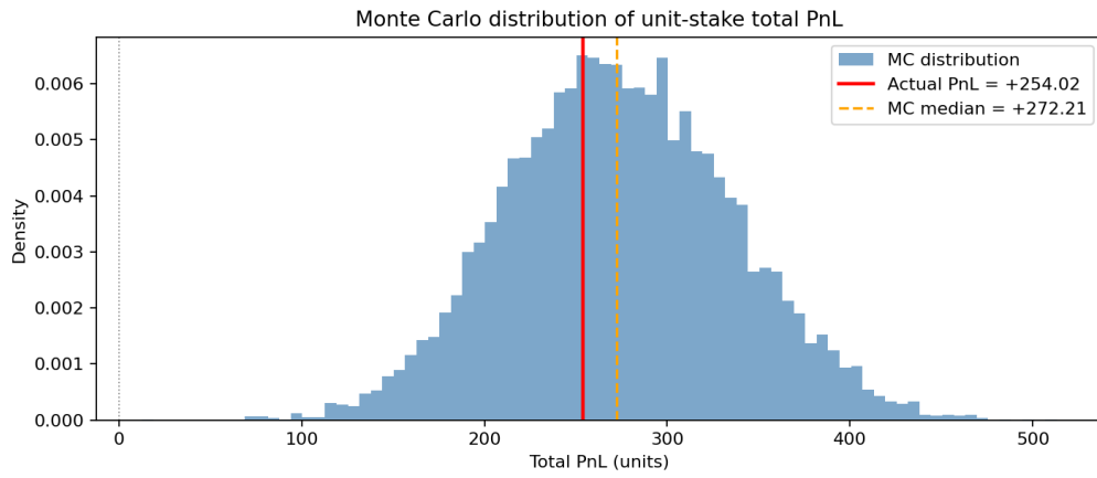
Figure 4: Monte Carlo distribution of unit-stake total PnL for the selected partition-B bets. This checks whether the model edge that feeds Kelly is believable.
