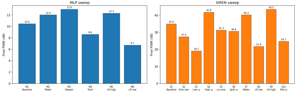
Figure 19: MLP and SIREN sweep final PSNR
