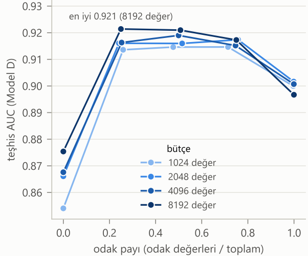
Göğüs röntgeni (COVID-QU-Ex), Model D
