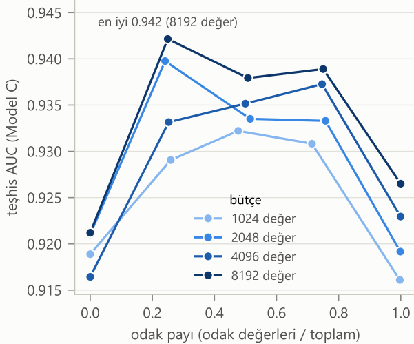
Göğüs röntgeni (COVID-QU-Ex), Model C
