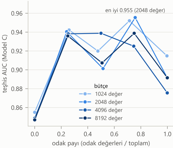
Göğüs röntgeni (COVID-QU-Ex), Model C
