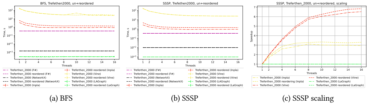
Figure 8: Evaluation results for Trefethen_2000 (both original and reoriented)
