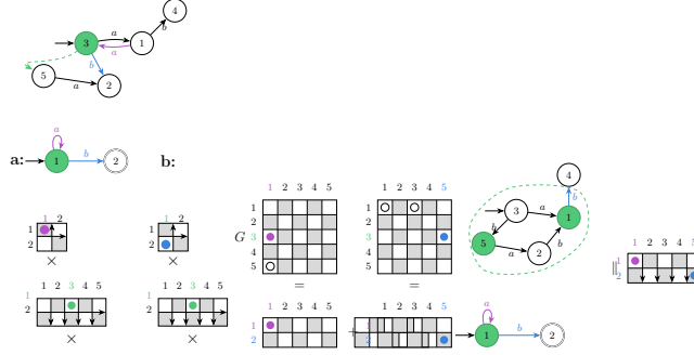
Fig. 5: Frontier update with path semantics: (a) simple paths filter, (b) trails filter.
