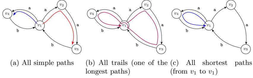
Fig. 1: Different query semantics for ((a^+)(b^?))^+
