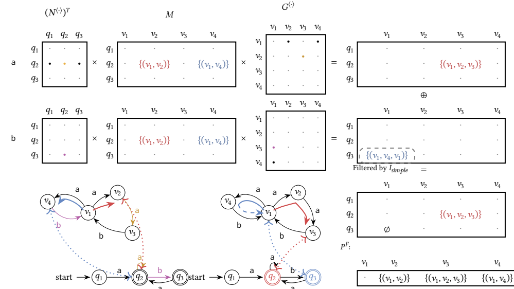
Figure 2: The algorithm step for graph and automaton for regular expression ((a^+)(b?))^+ using path semiring and all simple paths semantics
