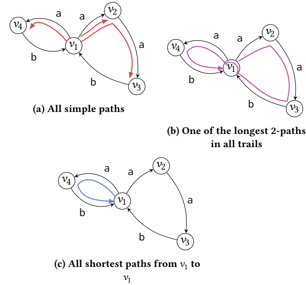
Figure 1: Different query semantics for ((a^+)(b?))^+
