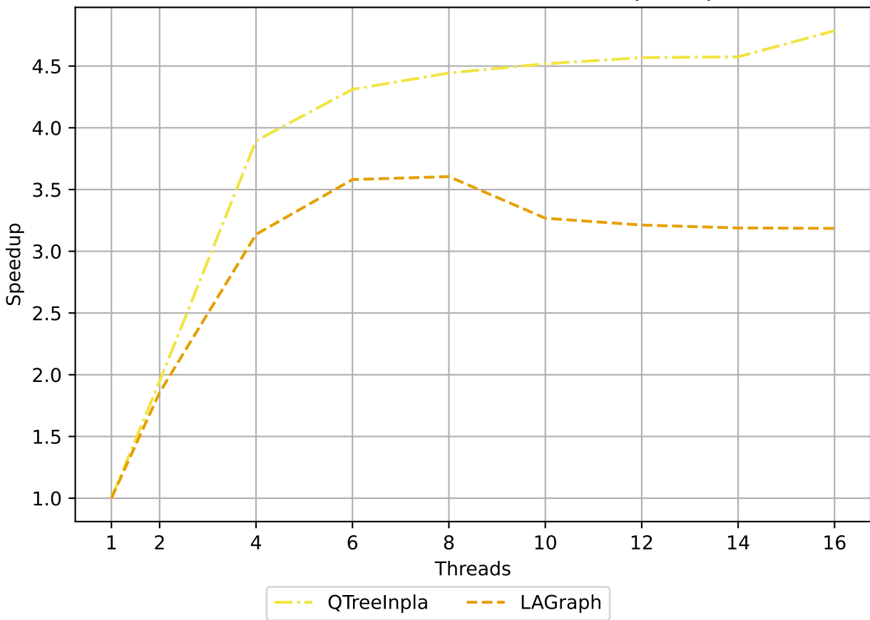
BFS, coAuthorCiteSeer, reordered, speedup
