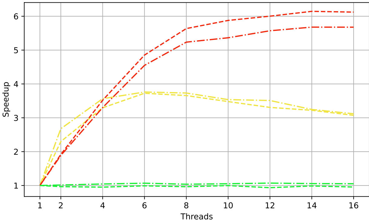
BFS, gr_30_30, un+reordered, scaling
