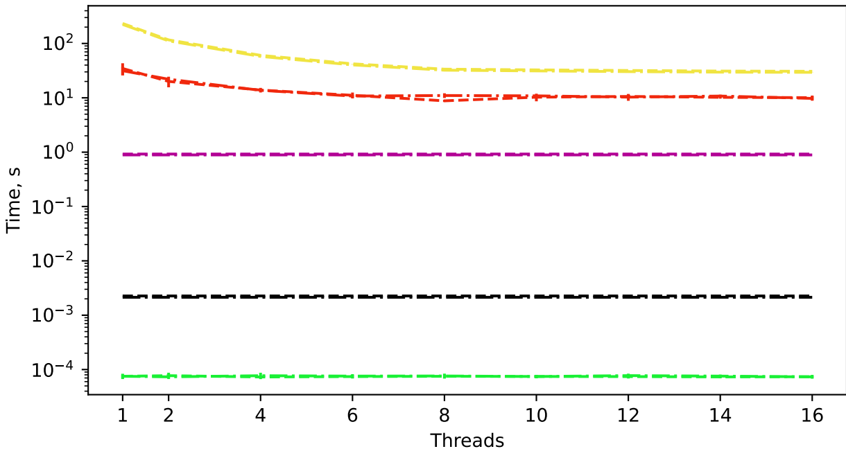
Triangle Counting, gr_30_30, un+reordered
