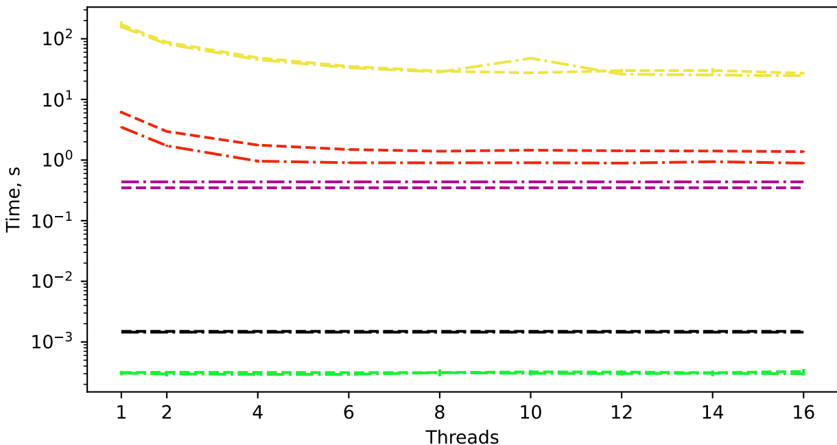
BFS, Trefethen2000, un+reordered
