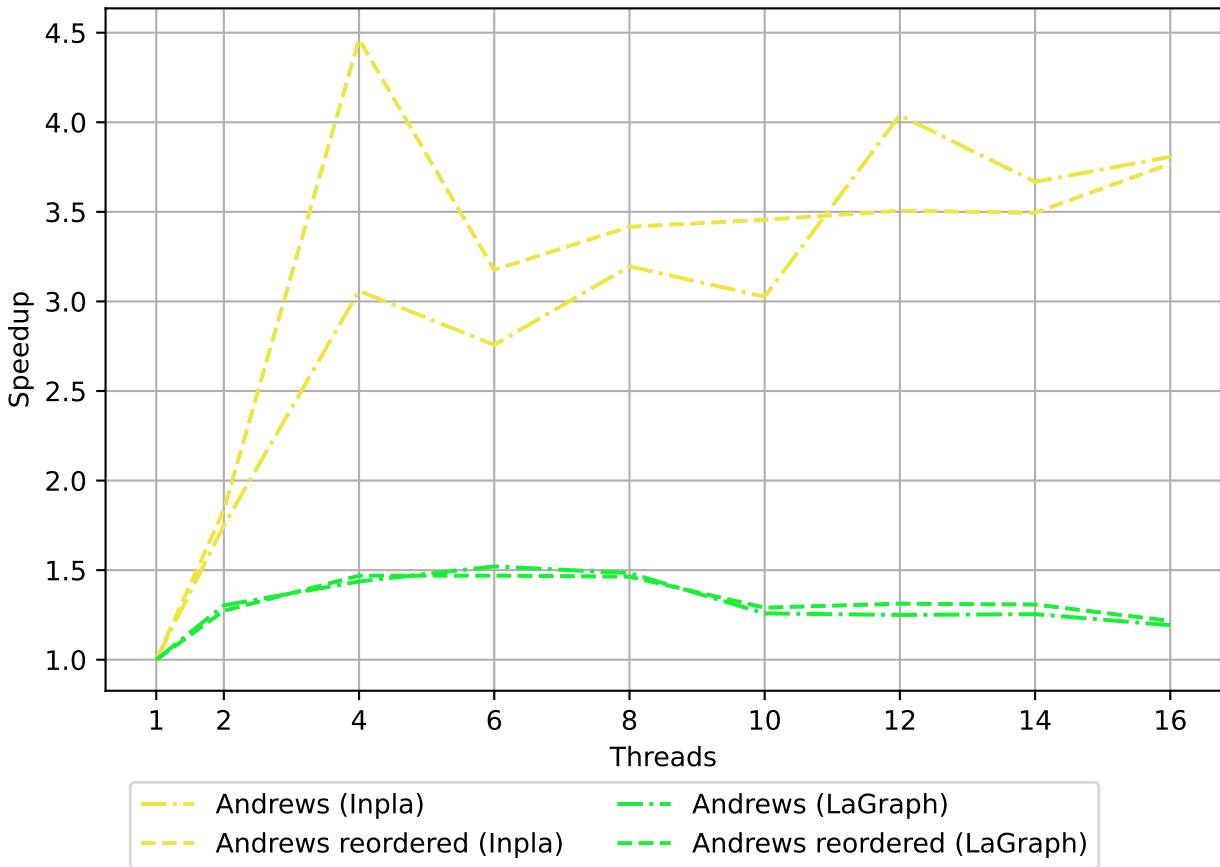
SSSP, Andrews, un+reordered, scaling
