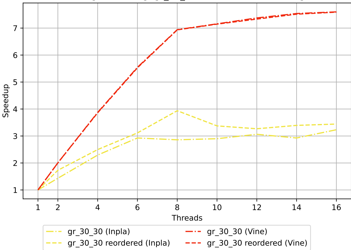
Triangle counting, gr_30_30, un+reordered, scaling
