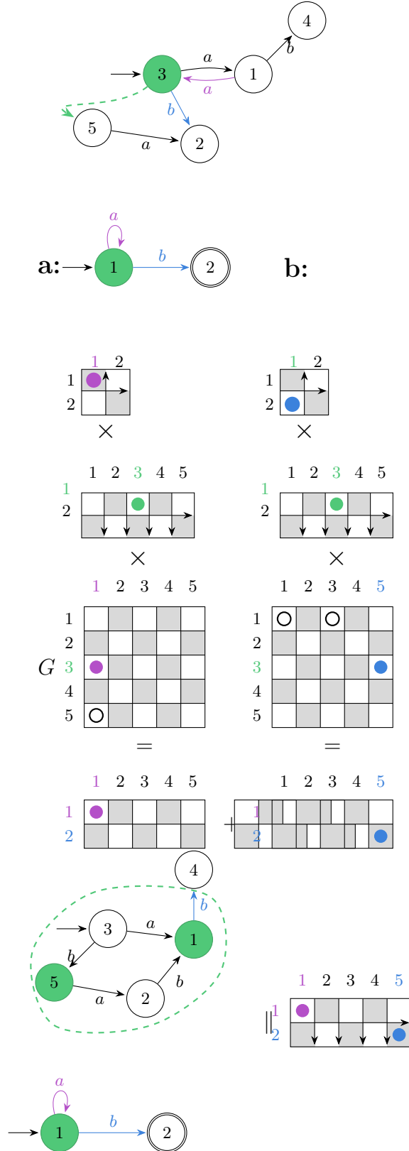
Fig. 4. Frontier update with path semantics: (a) simple paths filter, (b) trails filter.
