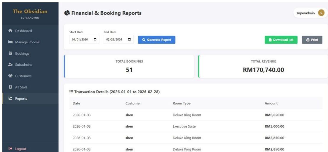
Figure 25 Reports
