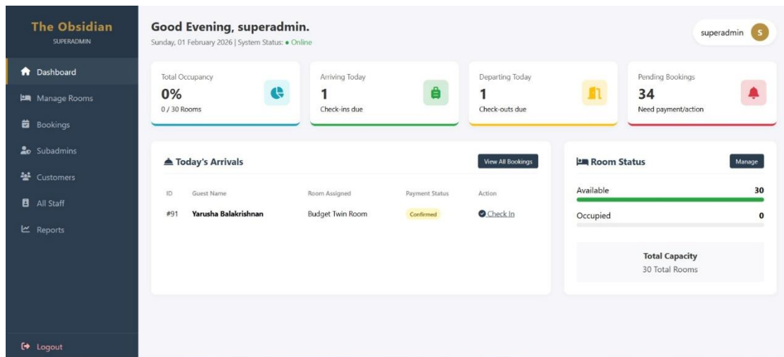
Figure 13 Admin Dashboard
