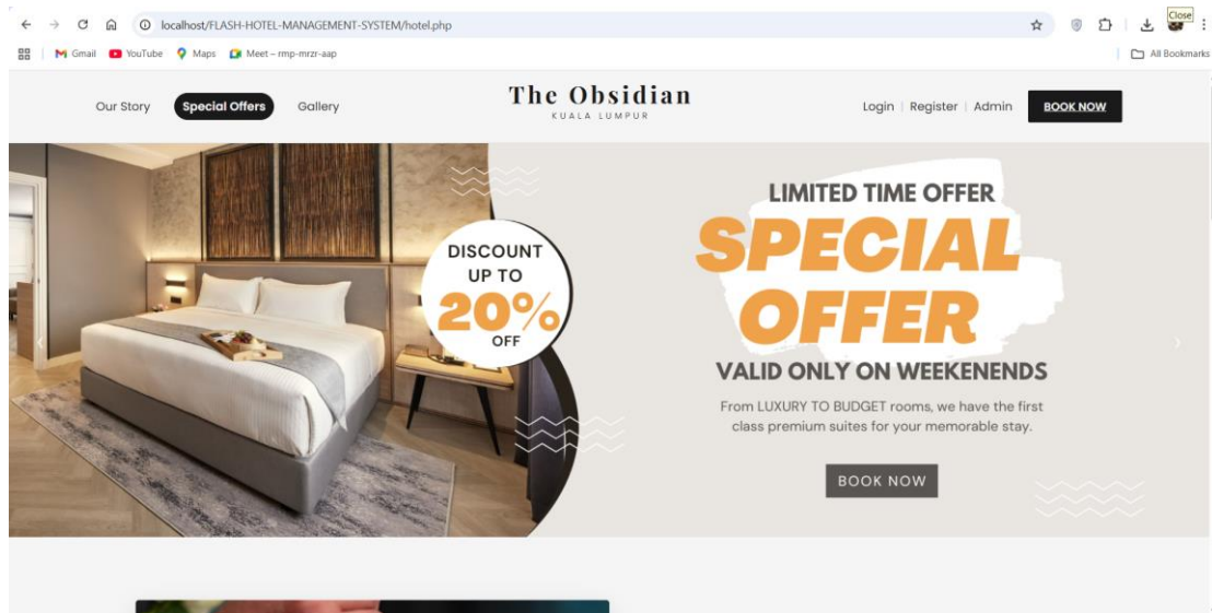
Figure 11 Customer dashboard
