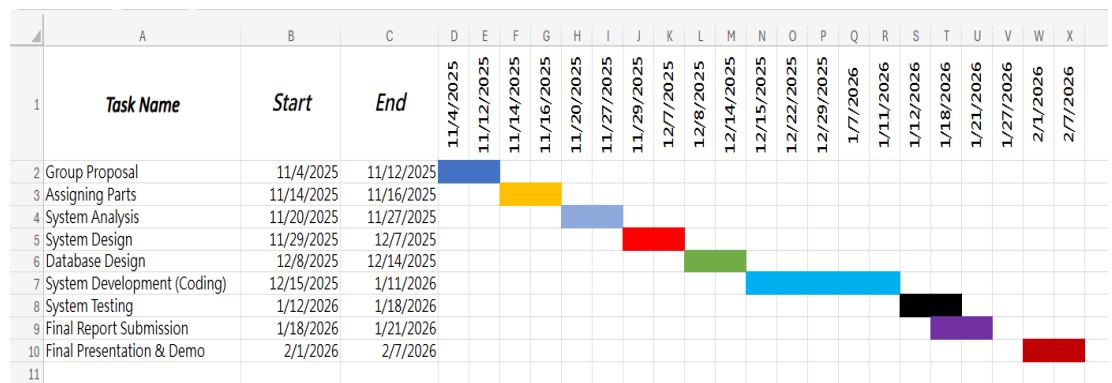
Figure 1:Gantt Chart
