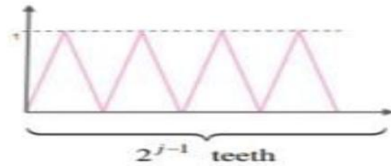
Figure 3: sawtooth function
