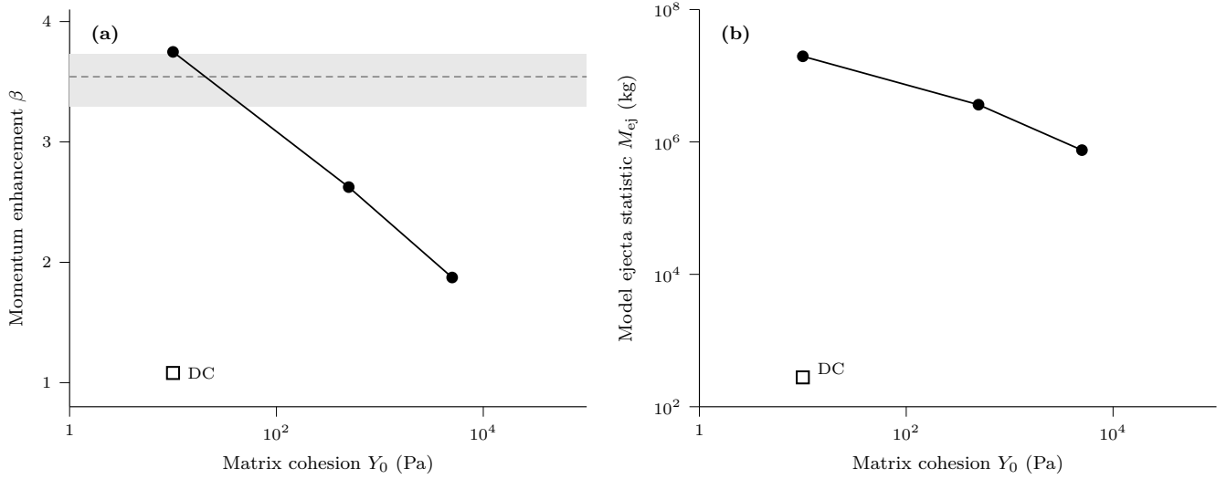
Figure 1. Controlled pilot measurements in the fixed DART scene. Filled circles and connecting segments show only the three completed cohesion runs; the segments are visual guides, not an inferred curve. The open square is the single matrix-tension comparison DC at 10 Pa. The gray band in the left panel is the mass-adjusted DART 1\sigma interval from Equation 1; the dashed line is its central value. The right panel shows the model-reported ejecta statistic, with no observational band because the LICIAcube plume estimate is not the same quantity. DN is omitted from the Y_0 sweep because it changes impact location.
