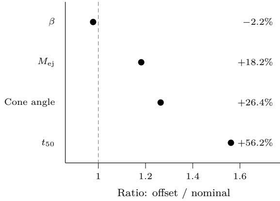
Figure 3. Impact-site sensitivity in the DY2–DN pair. Each marker is the 25 m offset result divided by the nominal result; the dashed line is unity. The percentages are changes relative to DY2, and the quantities are normalized only for visual comparison.
