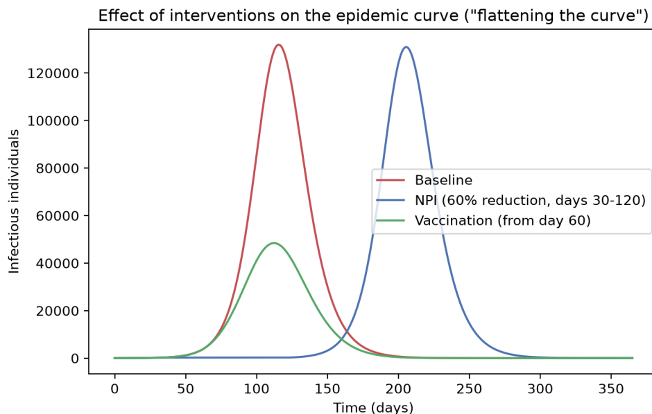
Figure 2. Infectious compartment (absolute count) over time across the three scenarios, illustrating that the temporary NPI shifts the peak in time without materially reducing its height, whereas vaccination reduces peak height directly.
