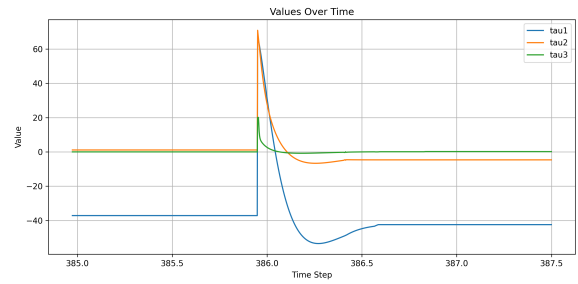
Figure 6: Applied torques \tau^* for jgotoControl with Kp values: q_1 = 600 , q_2 = 400 , q_3 = 200 , and Kv values: q_1 = 100 , q_2 = 40 , q_3 = 40 .
