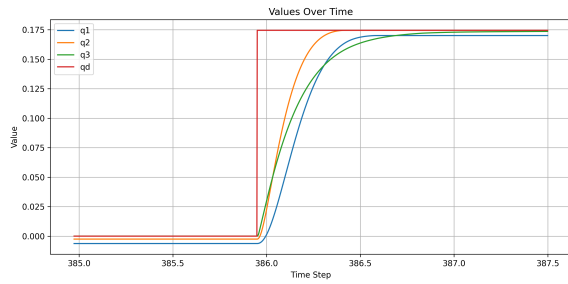
Figure 5: Desired joint states q_d^* and actual joint states q^* for jgotoControl with Kp values: q_1 = 600 , q_2 = 400 , q_3 = 200 , and Kv values: q_1 = 100 , q_2 = 40 , q_3 = 40 .
