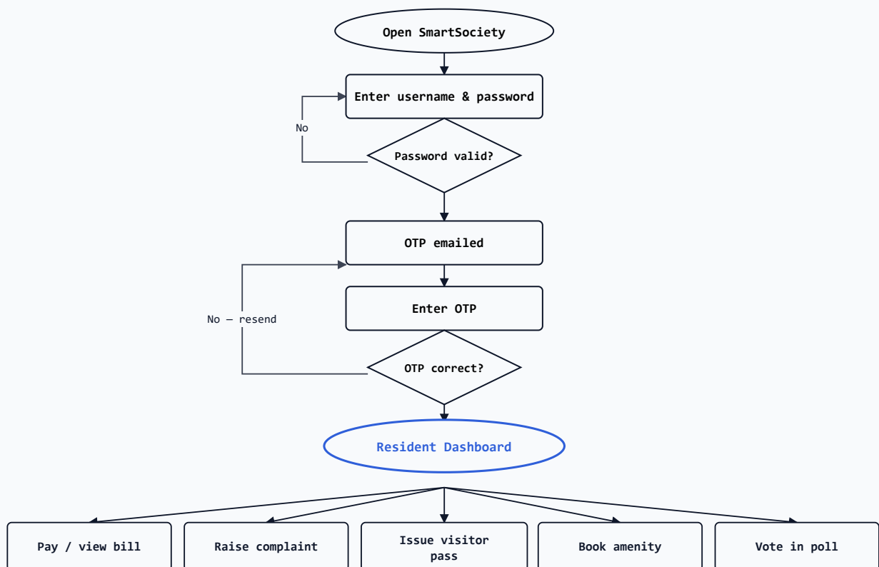
Fig. 1 – two-step OTP login, then five self-service actions the resident can take in any order. Paying a bill also offers a PDF receipt download; issuing a pass generates a QR/code shared with the guest.
