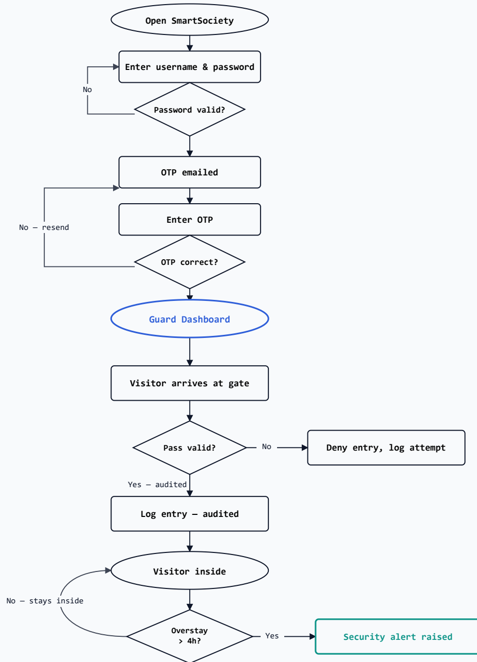
Fig. 3 – the overstay check runs as a repeating background job, not something the guard has to remember. Exit logging and the emergency-siren trigger are also available from the dashboard at any point; omitted here to keep the gate-decision loop legible.
