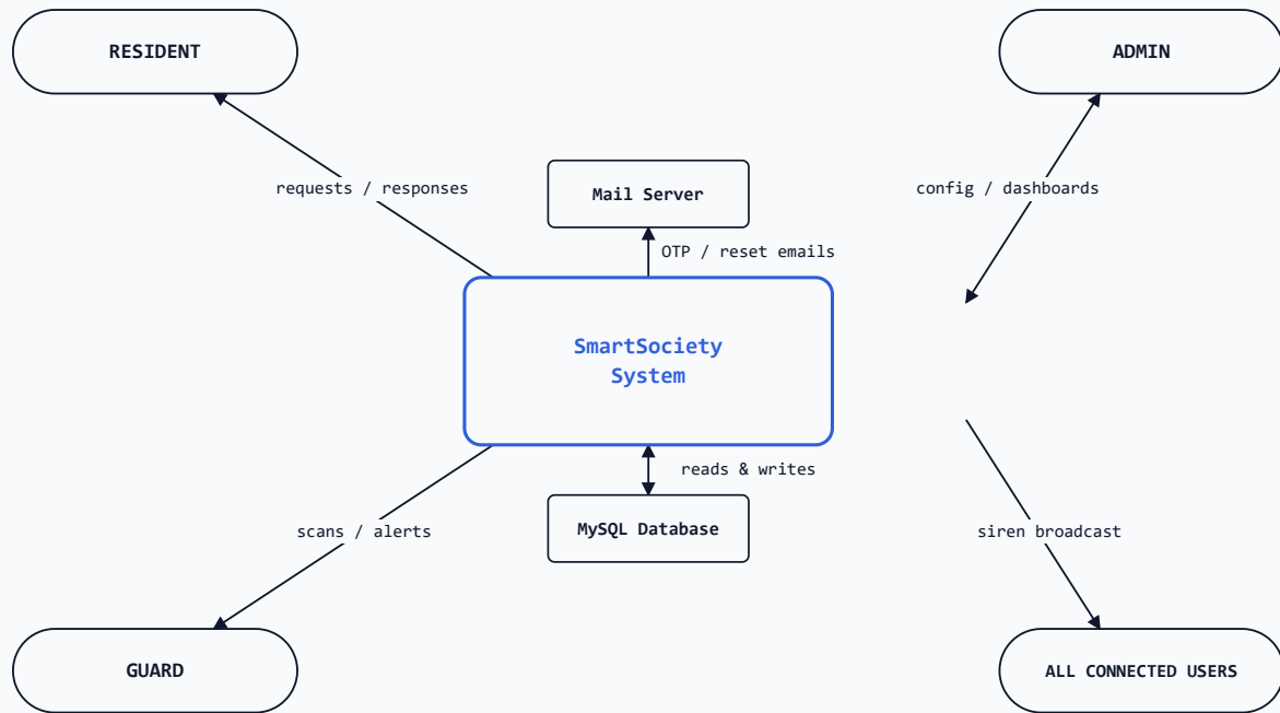
Fig. 4 – the whole application collapses to one process bounded by five external entities.
