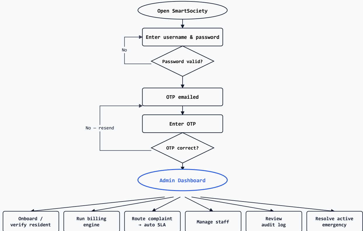
Fig. 2 – six independent oversight actions from one dashboard. Audit log review reads from the same trigger-protected table every financial edit and status change writes to (see Database Design §3).
