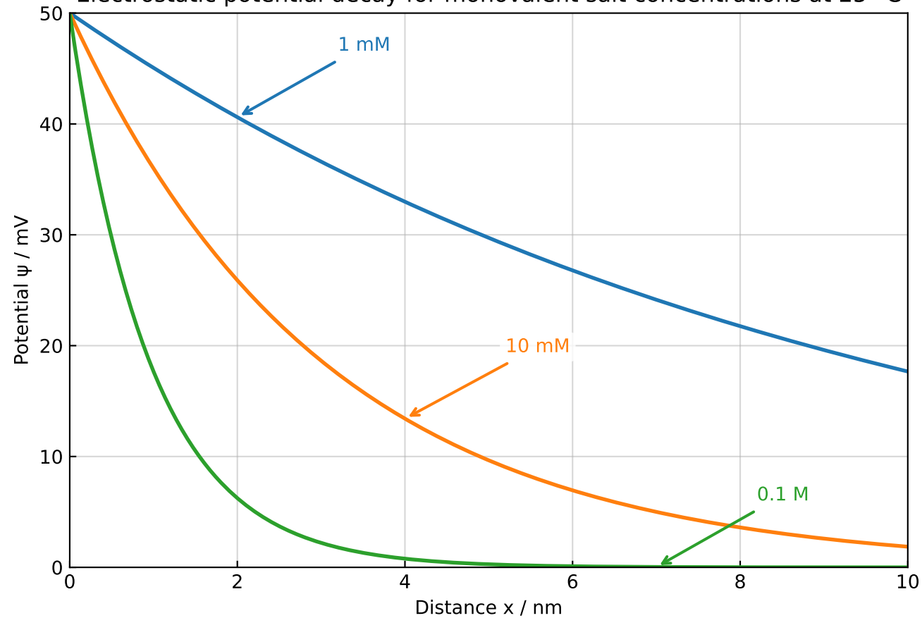
Electrostatic potential decay for monovalent salt concentrations at 25 °C
