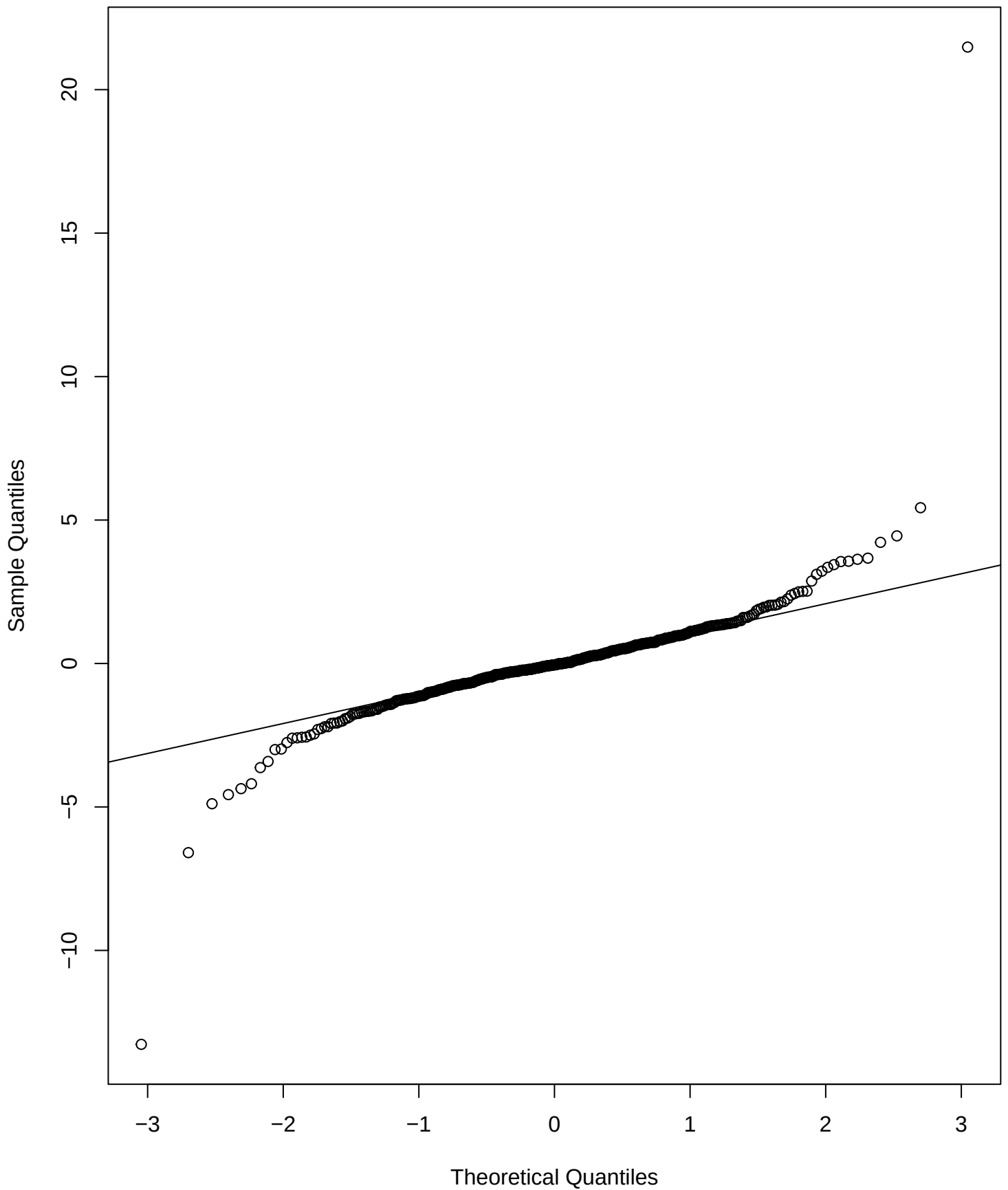
Normal Q-Q Plot
