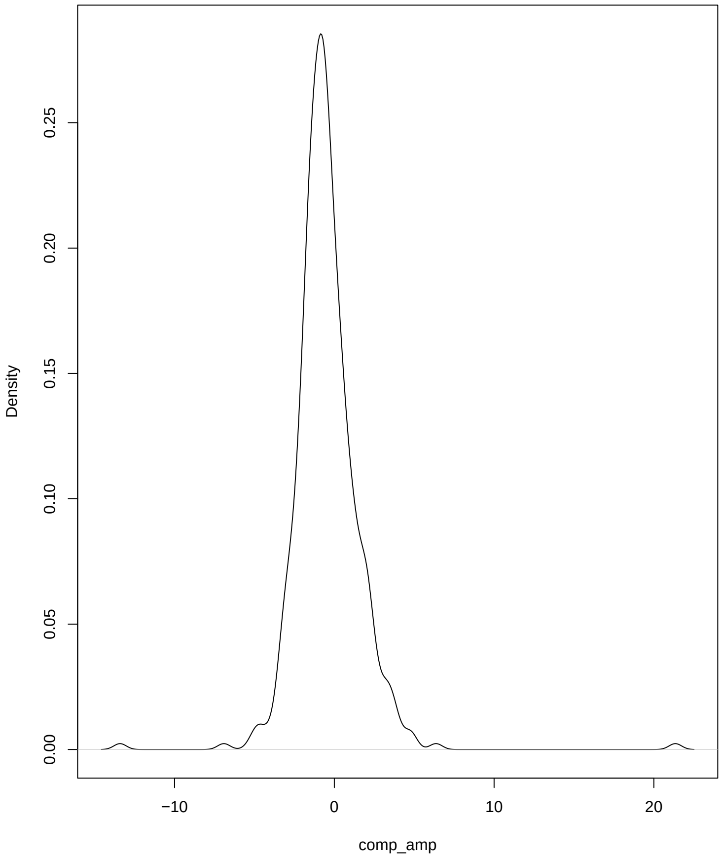
Density of comp_amp
