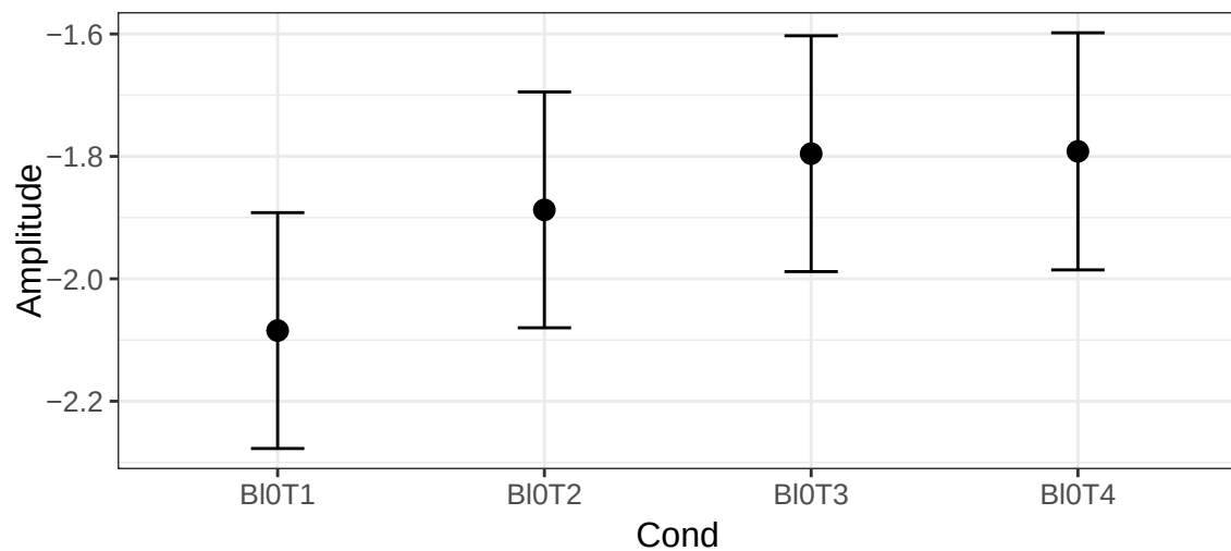
Main Effect of Cond
