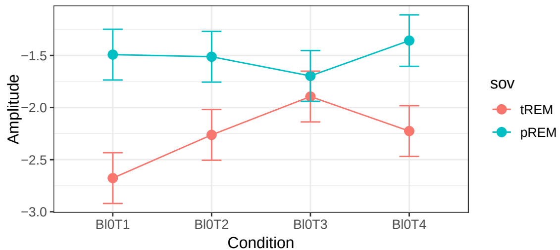
SOV x Condition Interaction
