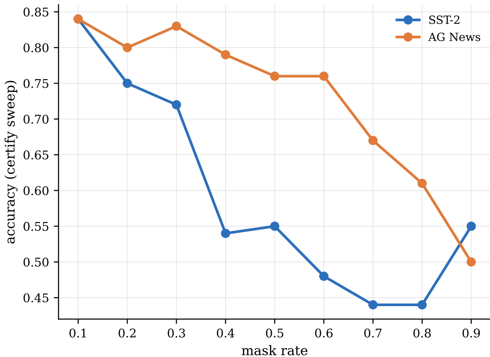
Accuracy vs mask rate
