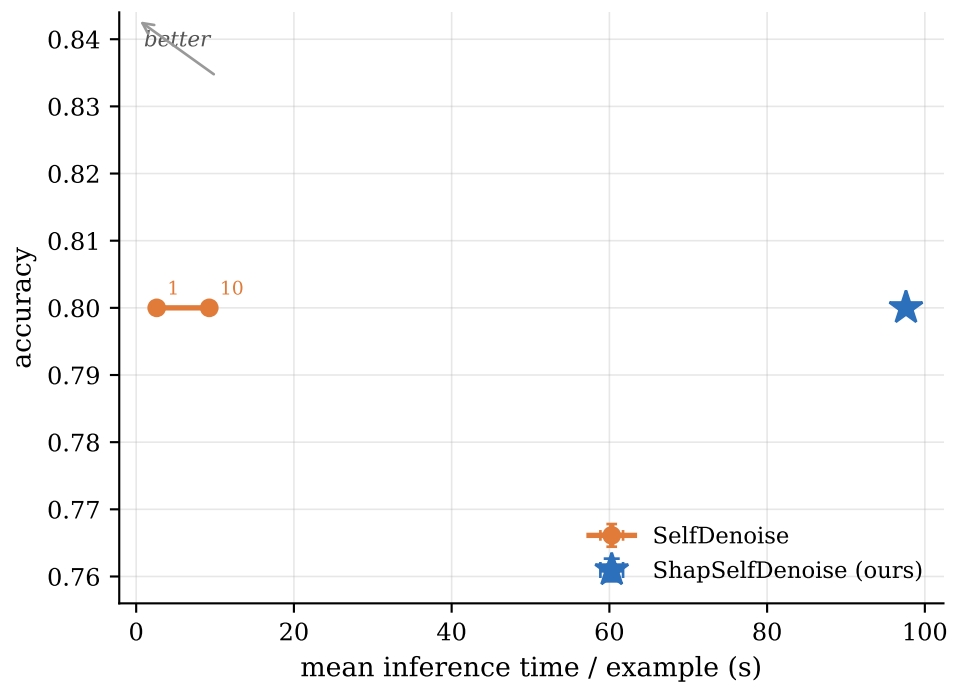
Accuracy vs inference time (numbers = SelfDenoise ensemble size)
