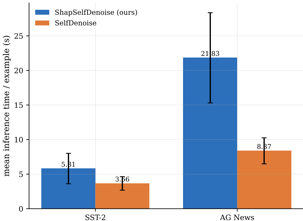
Per-example inference time
