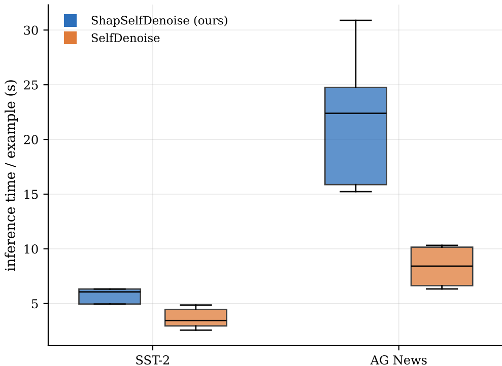
Inference-time distribution per example
