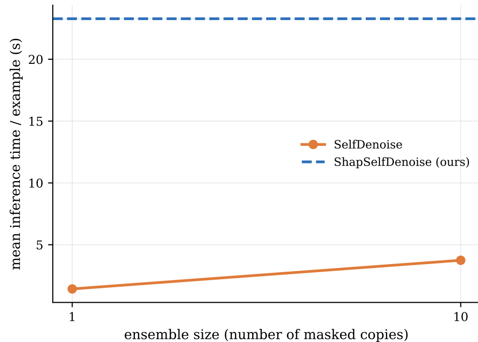
Inference time grows with the ensemble; ShapSelfDenoise is constant
