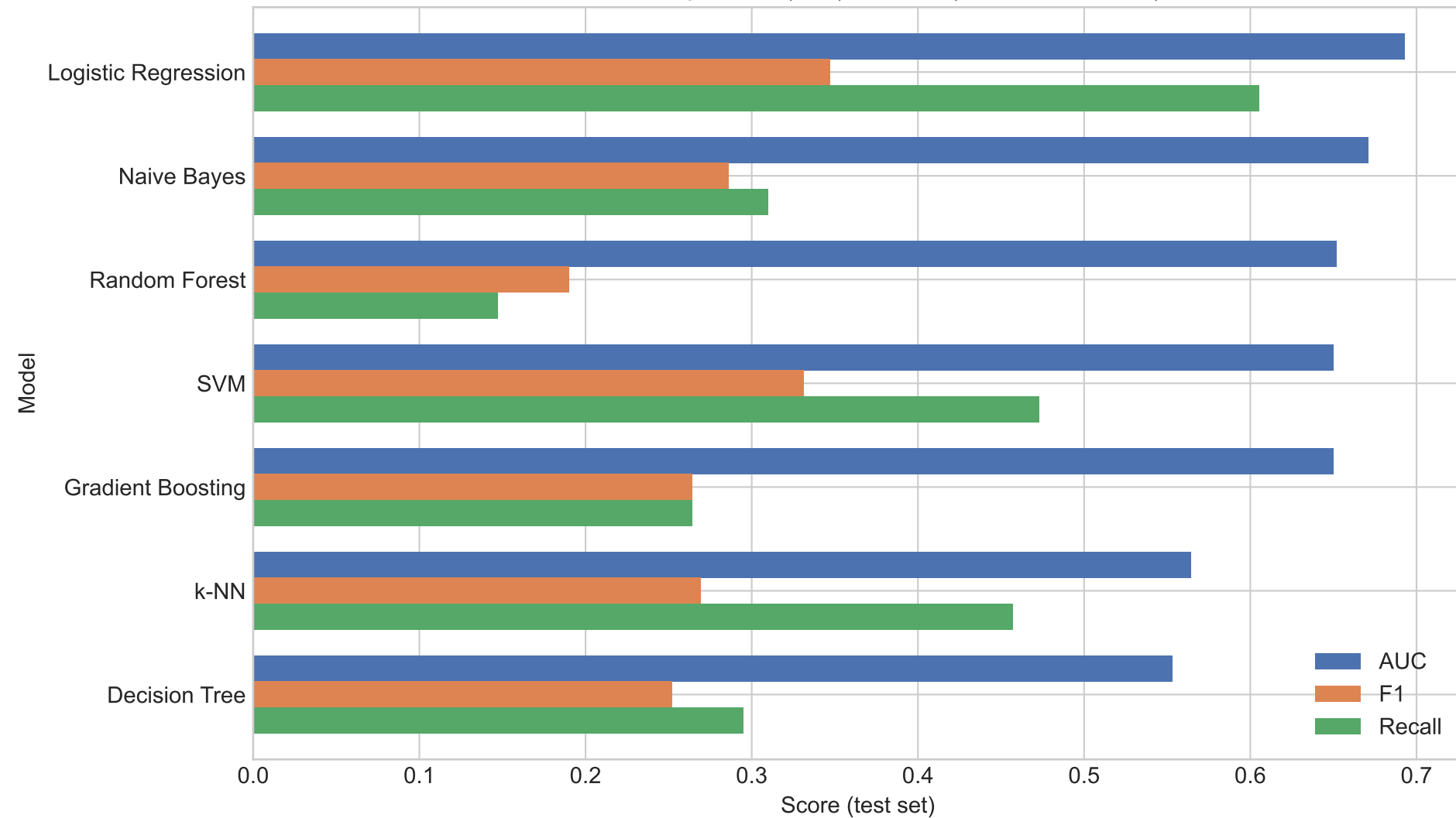
Model comparison (test) - scaled(AUC, F1, Recall)
