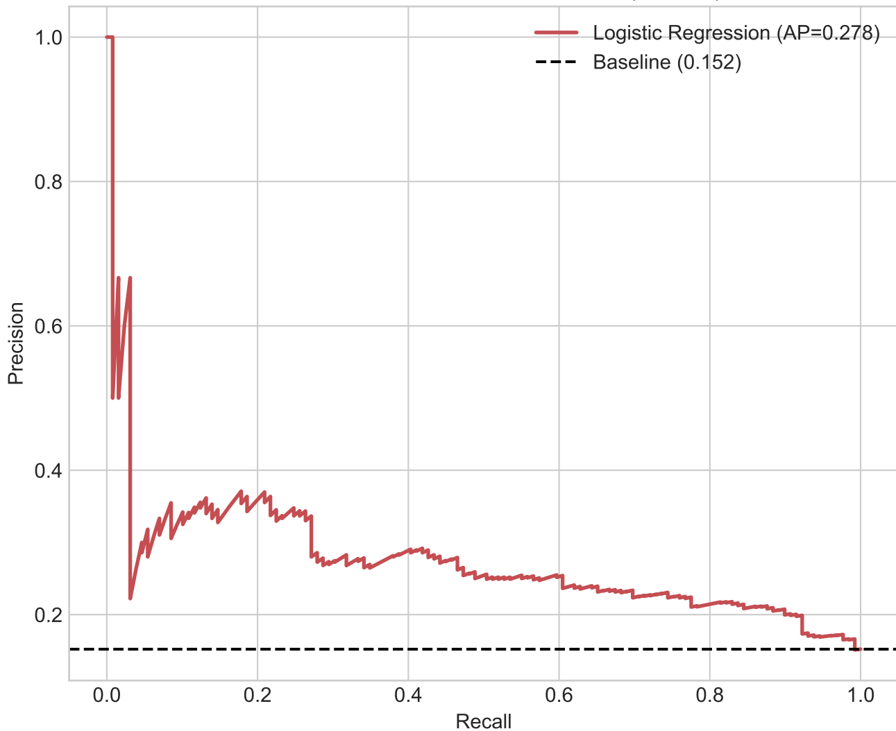
Final model Precision-Recall curve (test set)
