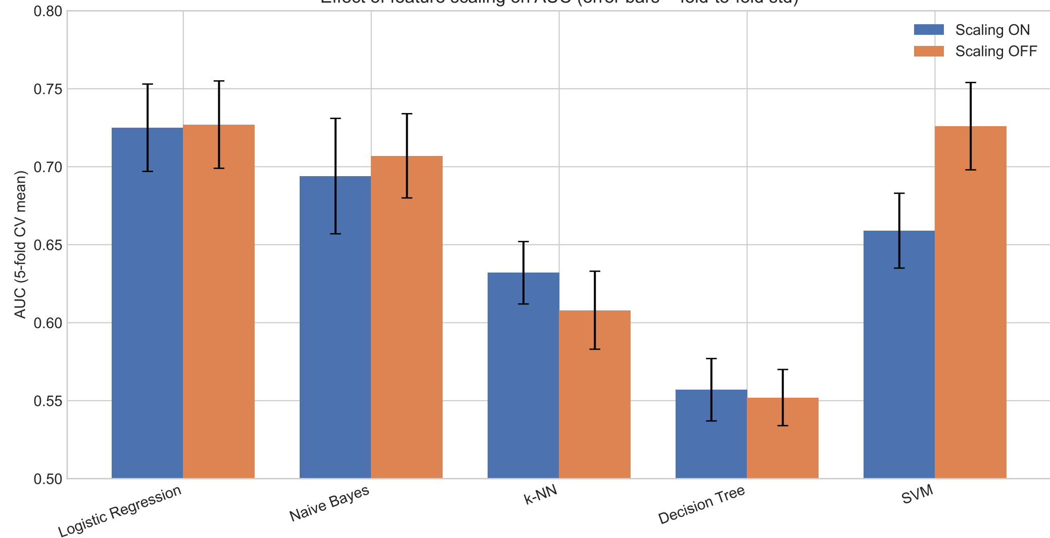
Effect of feature scaling on AUC (error bars = fold-to-fold std)
