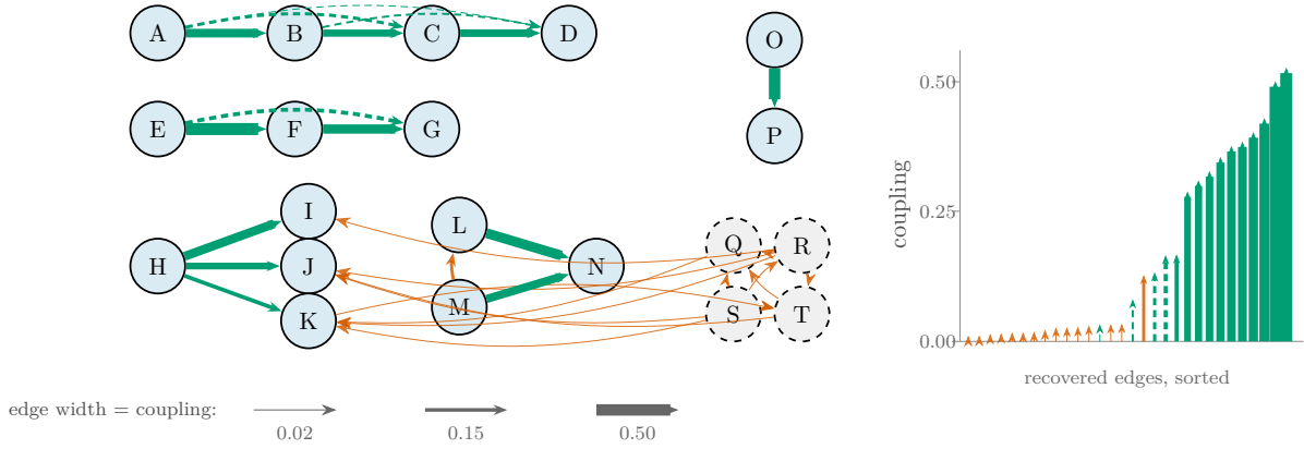
Figure 3: What cascadir recovered (one run: all , eff 0.30, t=6 ; 30 coupled pairs). Left: the method’s calls as a directed graph, oriented by cross_asym , on the Figure 1 layout; edge width = coupling strength (0.01–0.53; see scale). Green solid = an authored direct cascade recovered with correct direction (11/11); green dashed = a true indirect (transitive) coupling, e.g. A \rightarrow C via B (4); orange = a false-positive coupling (15); zero direct edges missed. Right: the same 30 edges as up-arrows sorted by coupling (both width and height encode coupling), keeping each edge’s colour and dash. The groups separate left-to-right: a hairline-short orange cluster (the isolated-negative over-call, at the noise floor), then green-dashed transitive links, then the tall, fat green direct cascades. The lone orange bar rising into the middle is M-L (a shared-downstream artifact — both drive N ), the only substantive false positive and the reason a plain coupling threshold cannot split true from false — which motivates a failure-mode analysis.
