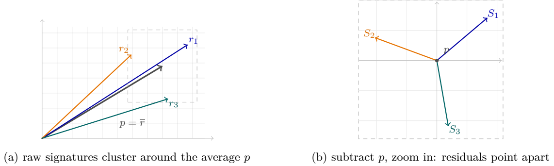
Figure 4: Panel-residualisation subtracts the shared program. (a) The raw signatures r_1, r_2, r_3 of three cytokines share a large common component and cluster around their average p = \bar{r} (grey), the shared-activation program; at this scale they are hard to tell apart. (b) We subtract the same vector p from each and zoom into the dashed box: the residual S_i = r_i - p is each cytokine’s deviation from the average. The residuals point in clearly different directions, so the cytokine-specific signatures become distinguishable; because they are deviations from a mean, they sum to zero. This residual is the signature carried downstream. The effect of the shared-activation confound on coupling is treated in Section 4.5.
