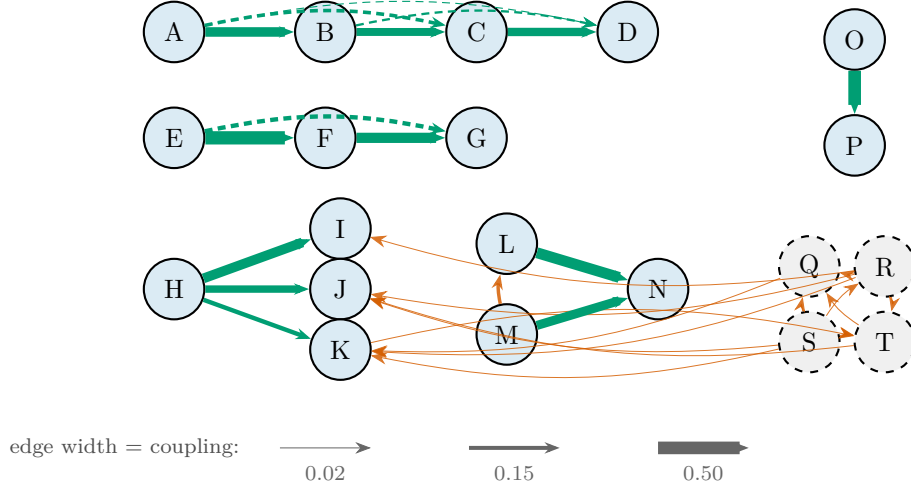
Figure 3: What cascadir recovered (one run: all , eff 0.30, t=6 ; 30 coupled pairs). Directed edges are the method’s calls, oriented by cross_asym , on the Figure 1 layout. Green solid : an authored direct cascade recovered with correct direction (11/11). Green dashed : a true but indirect (transitive) coupling, e.g. A \rightarrow C via B (4). Orange : a false-positive coupling with no cascade relationship (15). Edge width = coupling strength (range 0.01–0.53; see scale): the real cascades are the fat arrows, the isolated-negative over-call sits at the hairline noise floor, and the one substantive false positive, M-L (a shared-downstream artifact, both drive N ), is the visibly thicker orange edge. Zero authored direct edges were missed.
