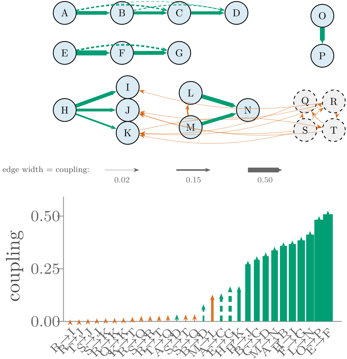
Figure 3: What cascadir recovered (one run: all, eff 0.30, t=6 ; 30 coupled pairs). Top: the method's calls as a directed graph oriented by cross_asym on the Figure 1 layout; edge width = coupling strength (0.01–0.53; see scale). Green solid = an authored direct cascade recovered with correct direction (11/11); green dashed = a true indirect (transitive) coupling, e.g. A \rightarrow C via B (4); orange = a false-positive coupling (15); zero direct edges missed. Bottom: the same 30 recovered edges, sorted by coupling strength.
