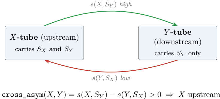
Figure 8: Why cross_asym encodes direction. The upstream tube engages the downstream signature more than vice versa; directional_score (symmetric) averages this away, cross_asym (antisymmetric) keeps it.
