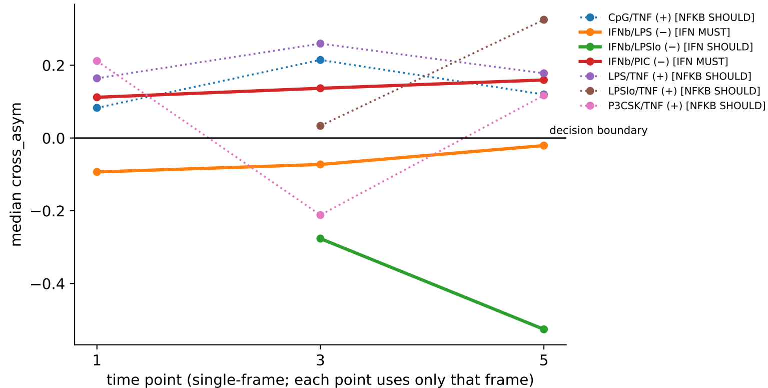
Sheu BMDM: cross_asym kinetics for the 7 benchmark cascades
