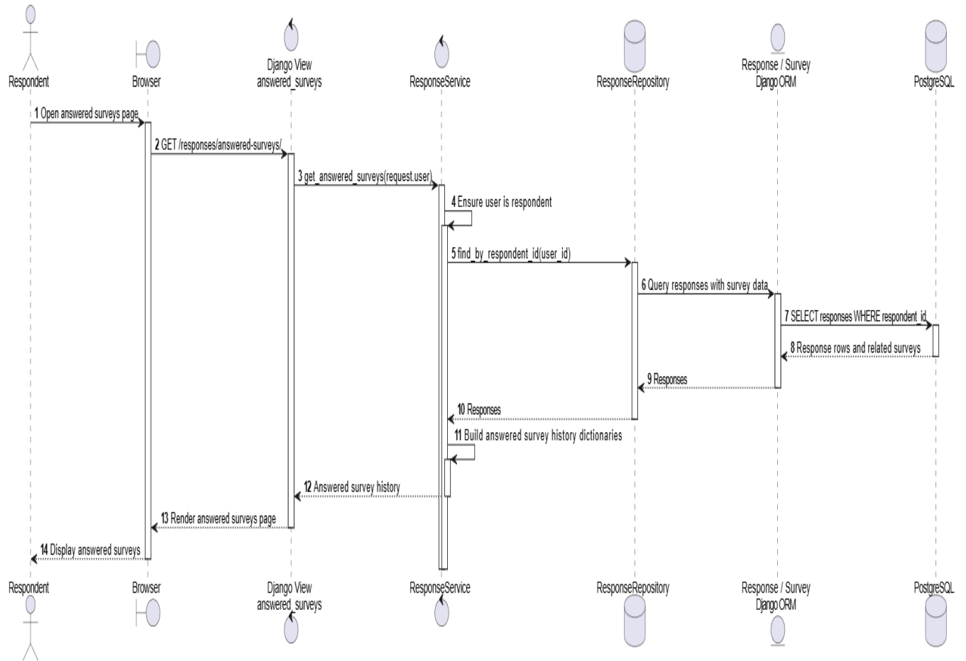
Sequence Diagram - UC-17 View Answered Surveys
