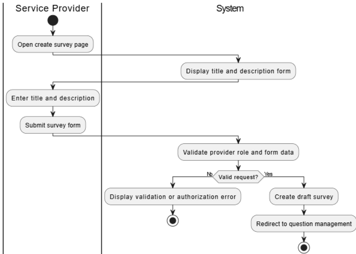
Activity Diagram - UC-05 Create Survey
