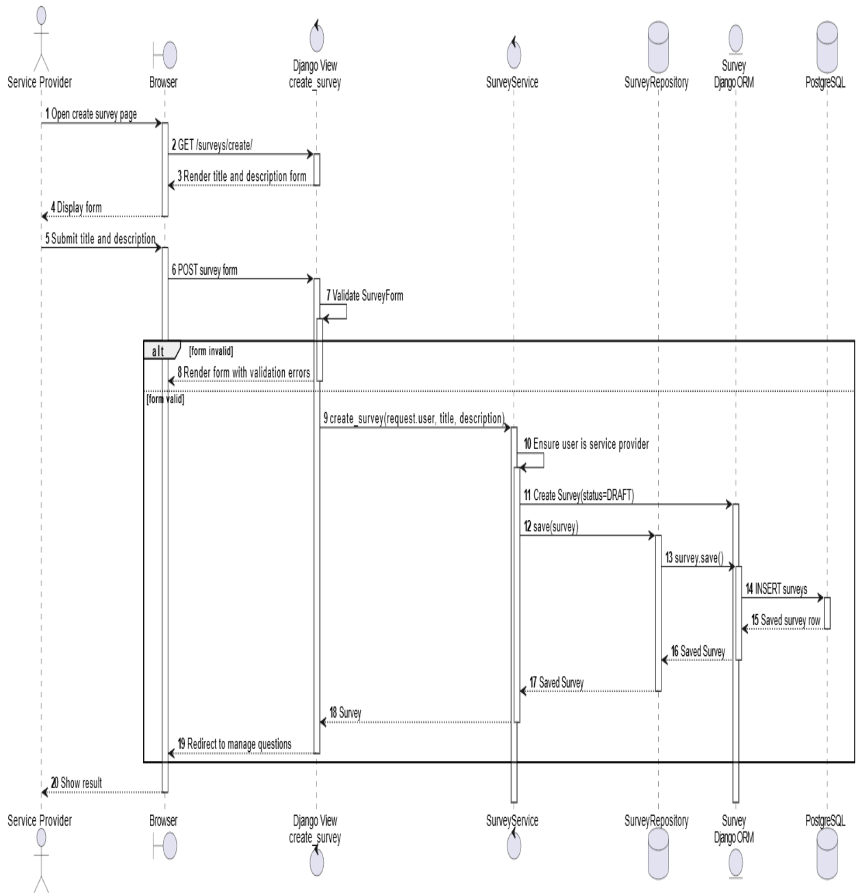
Sequence Diagram - UC-05 Create Survey
