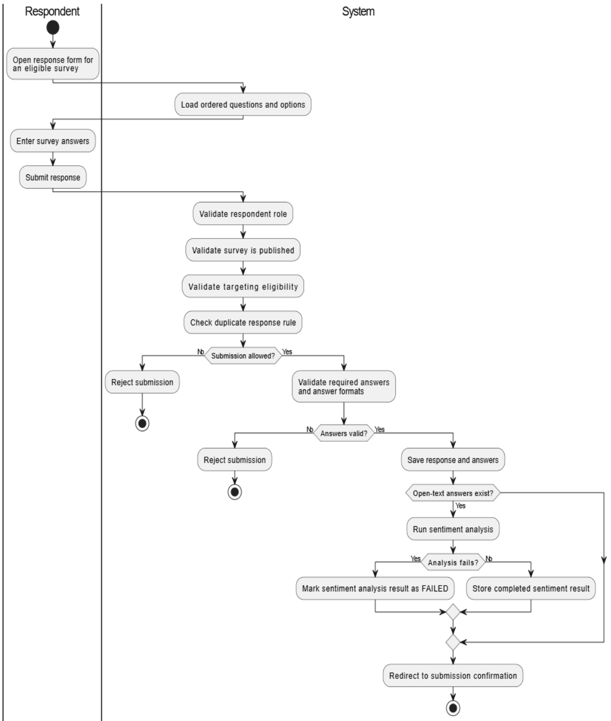
Activity Diagram - UC-16 Submit Survey Response
