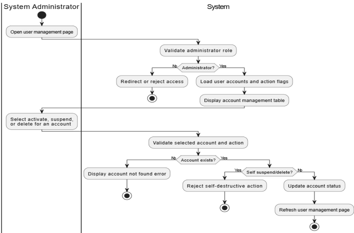
Activity Diagram - UC-18 Manage User Accounts
