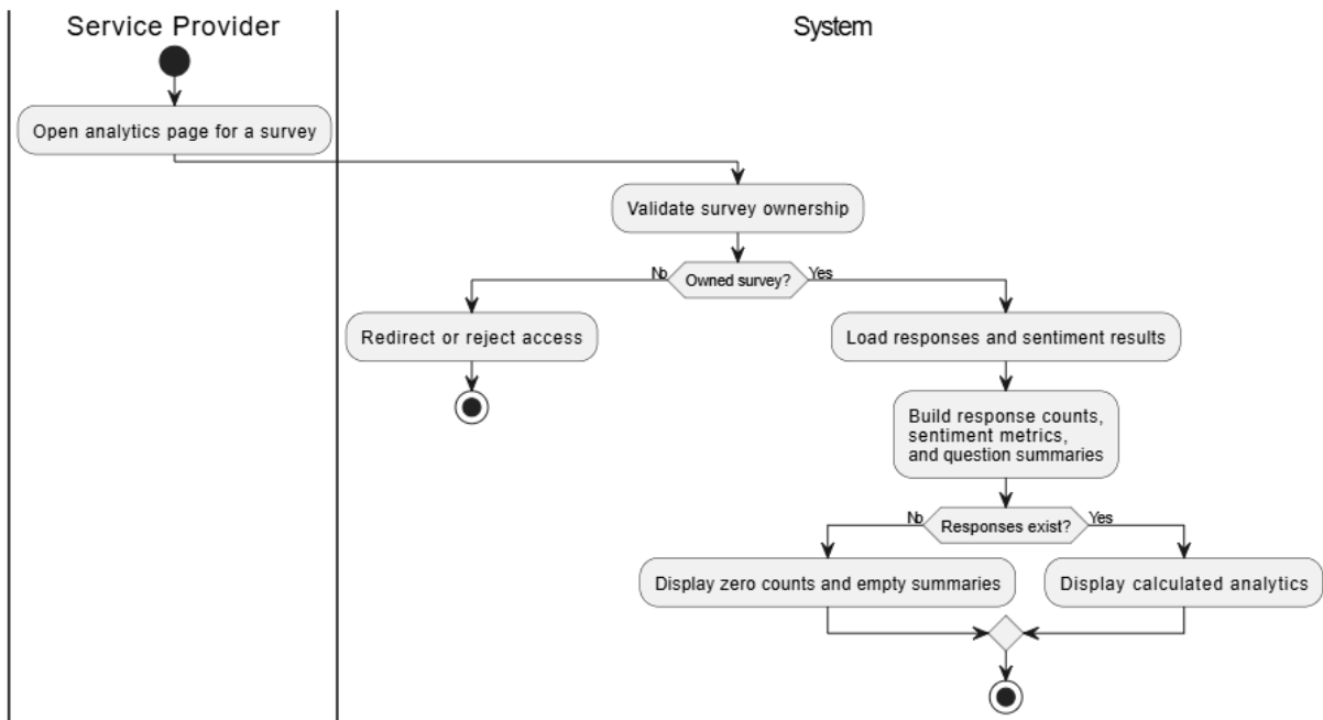
Activity Diagram - UC-13 View Analysis Results
