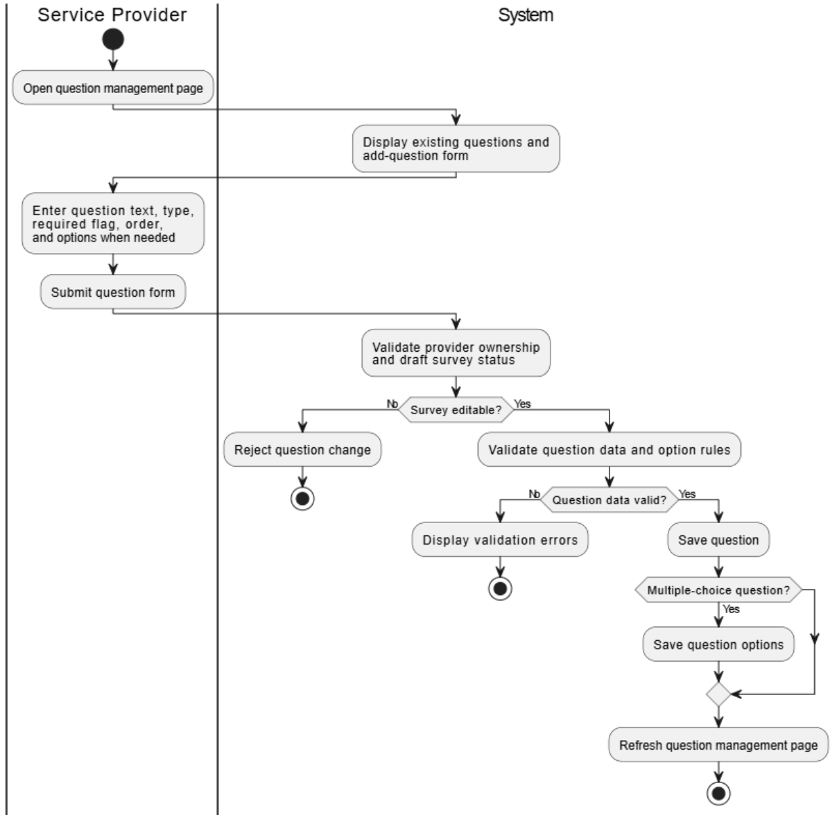
Activity Diagram - UC-08 Add Question
