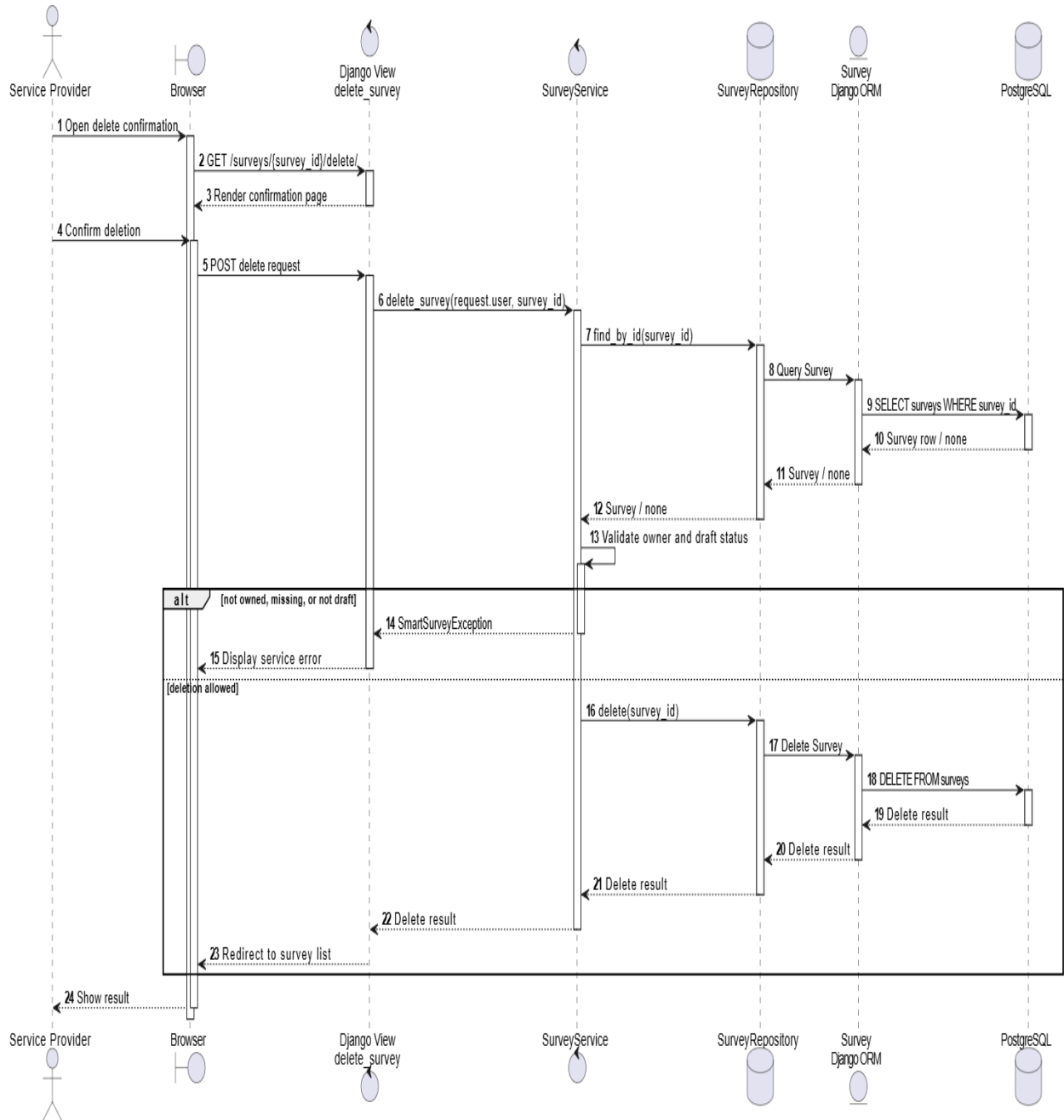
Sequence Diagram - UC-07 Delete Survey
