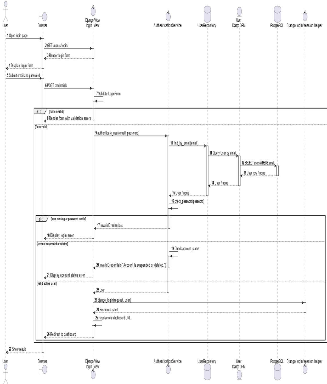
Sequence Diagram - UC-03 Login
