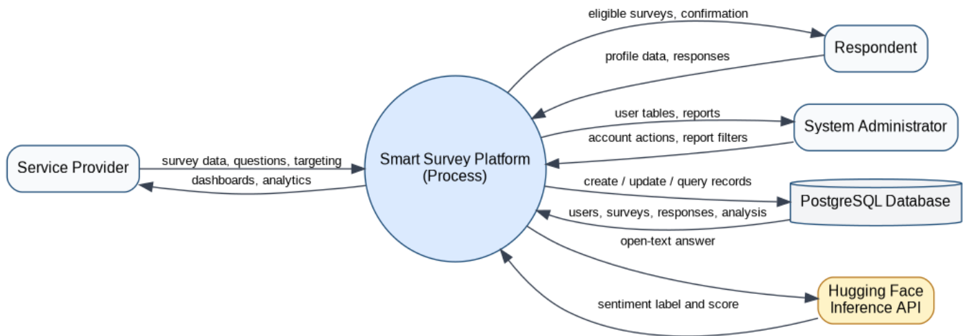
Figure B.7: DFD Level 0 for the Smart Survey Platform
