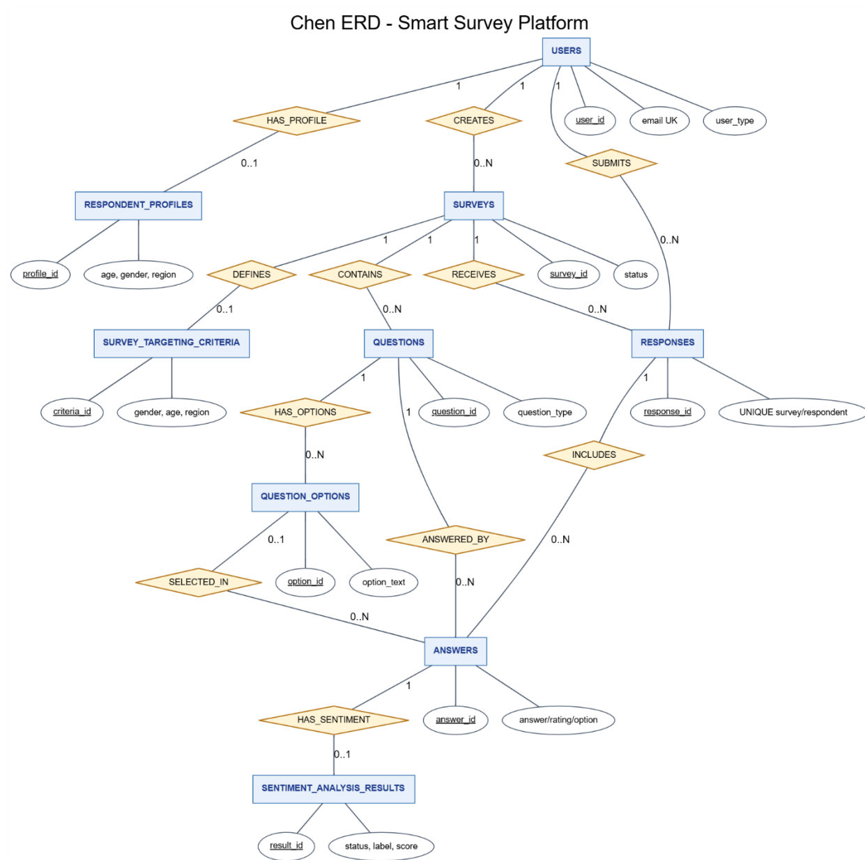
Figure B.3: Chen Entity Relationship Diagram
