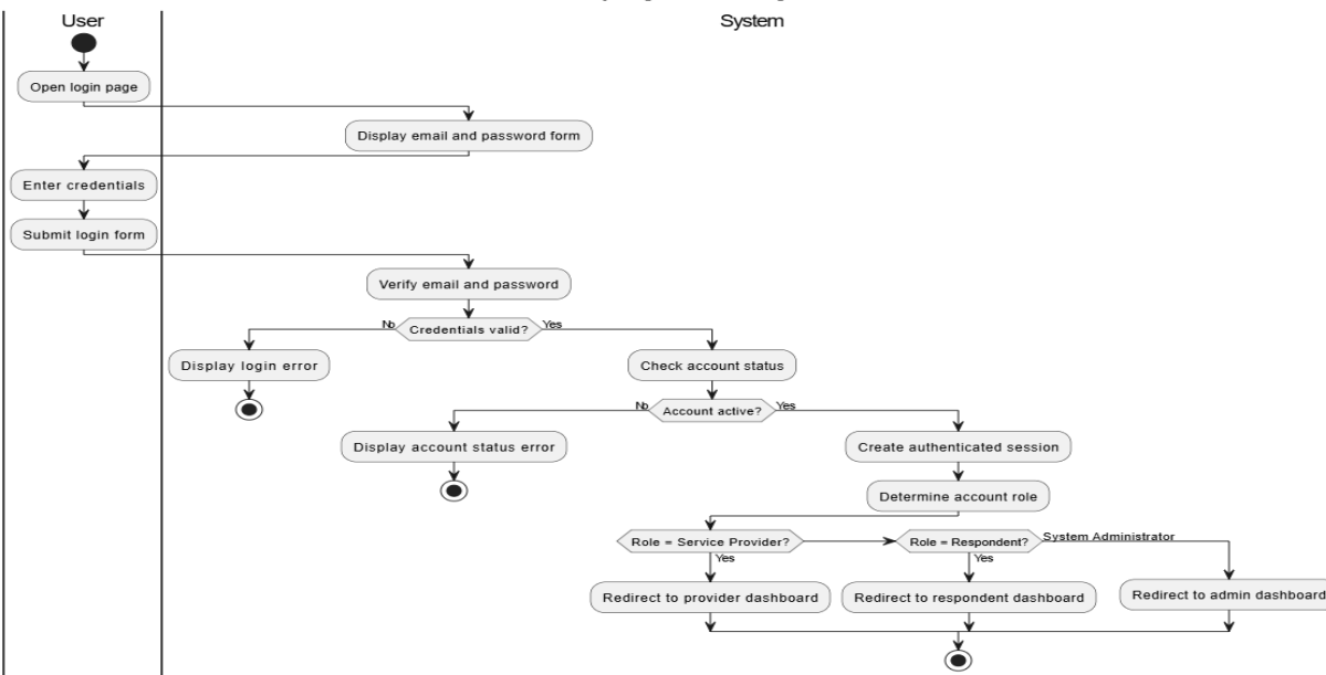
Activity Diagram - UC-03 Login
