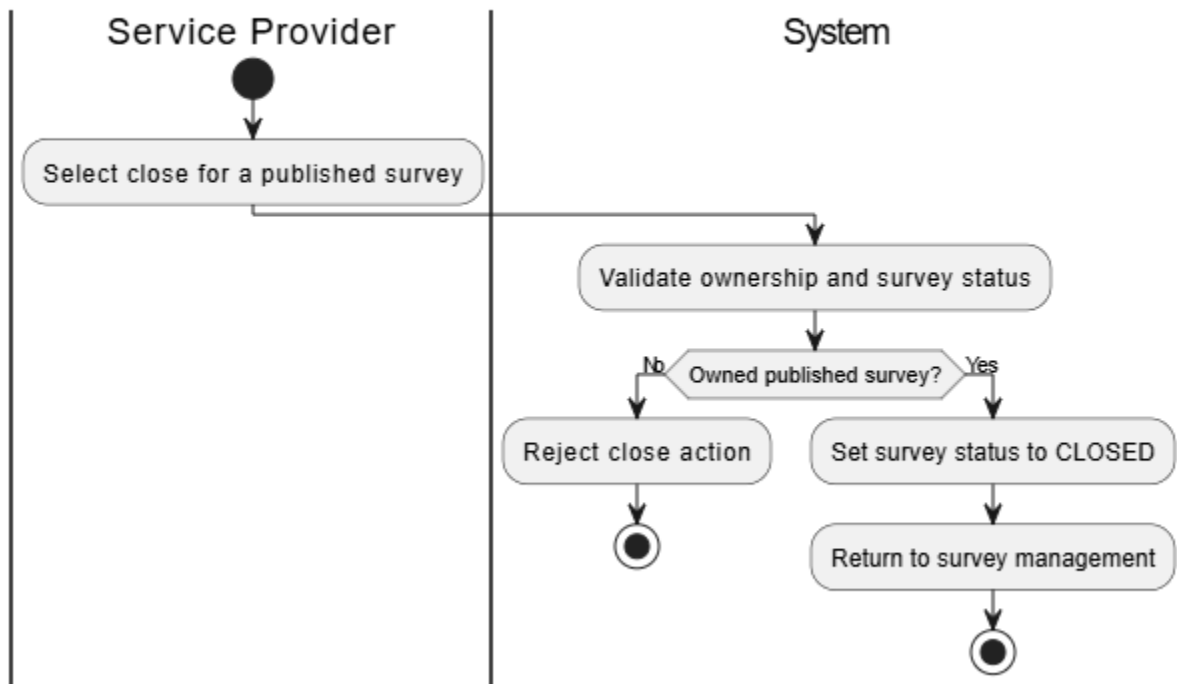
Activity Diagram - UC-12 Close Survey
