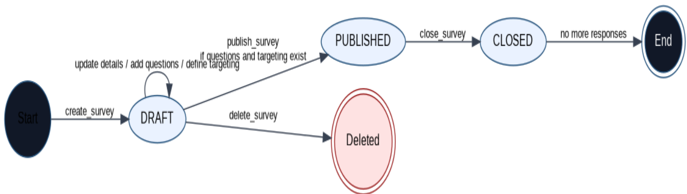
Figure B.8: State Machine Diagram for Survey Lifecycle
