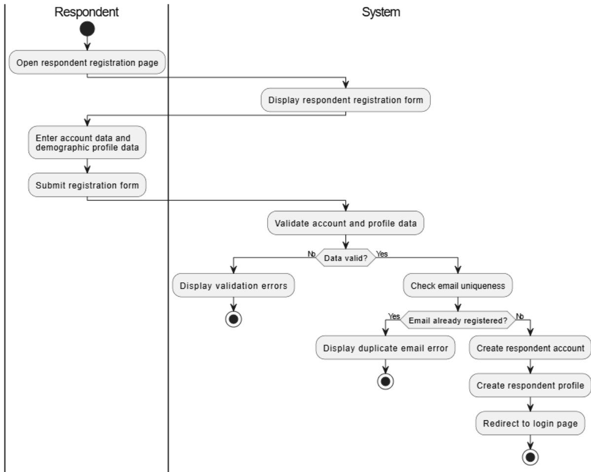
Activity Diagram - UC-02 Register as Respondent
