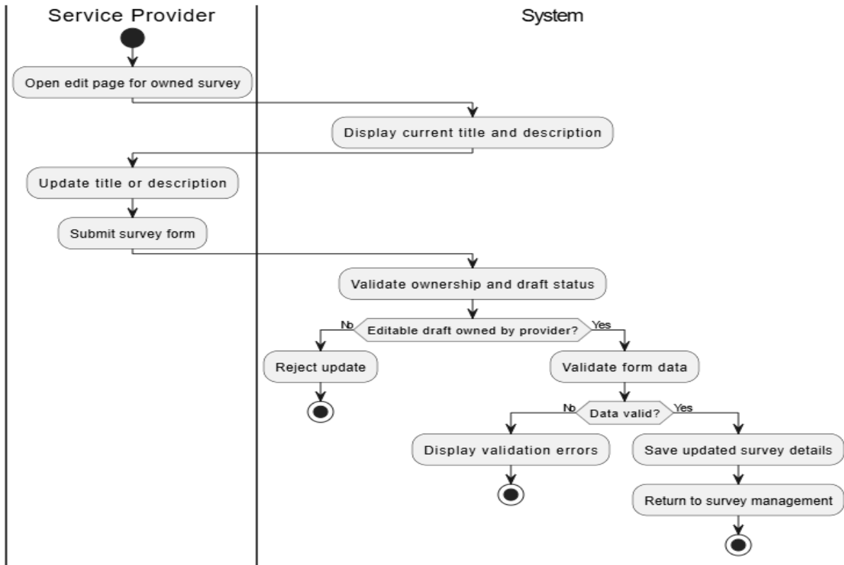
Activity Diagram - UC-06 Update Survey Details
