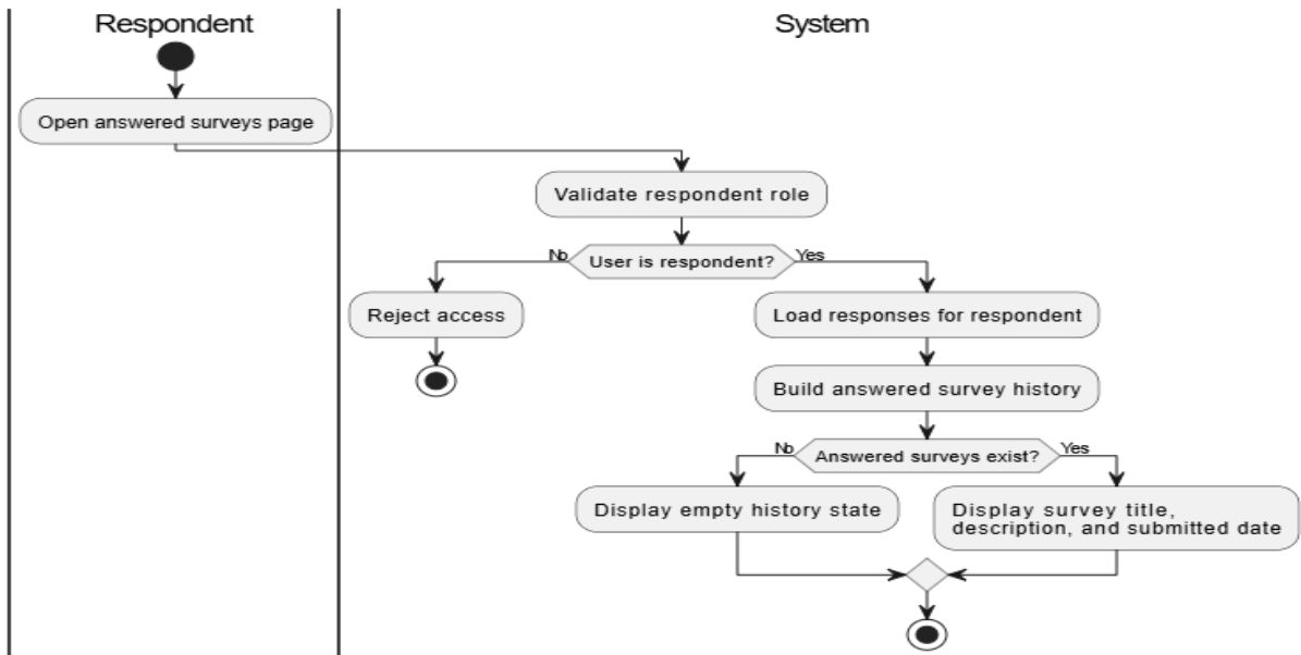
Activity Diagram - UC-17 View Answered Surveys
