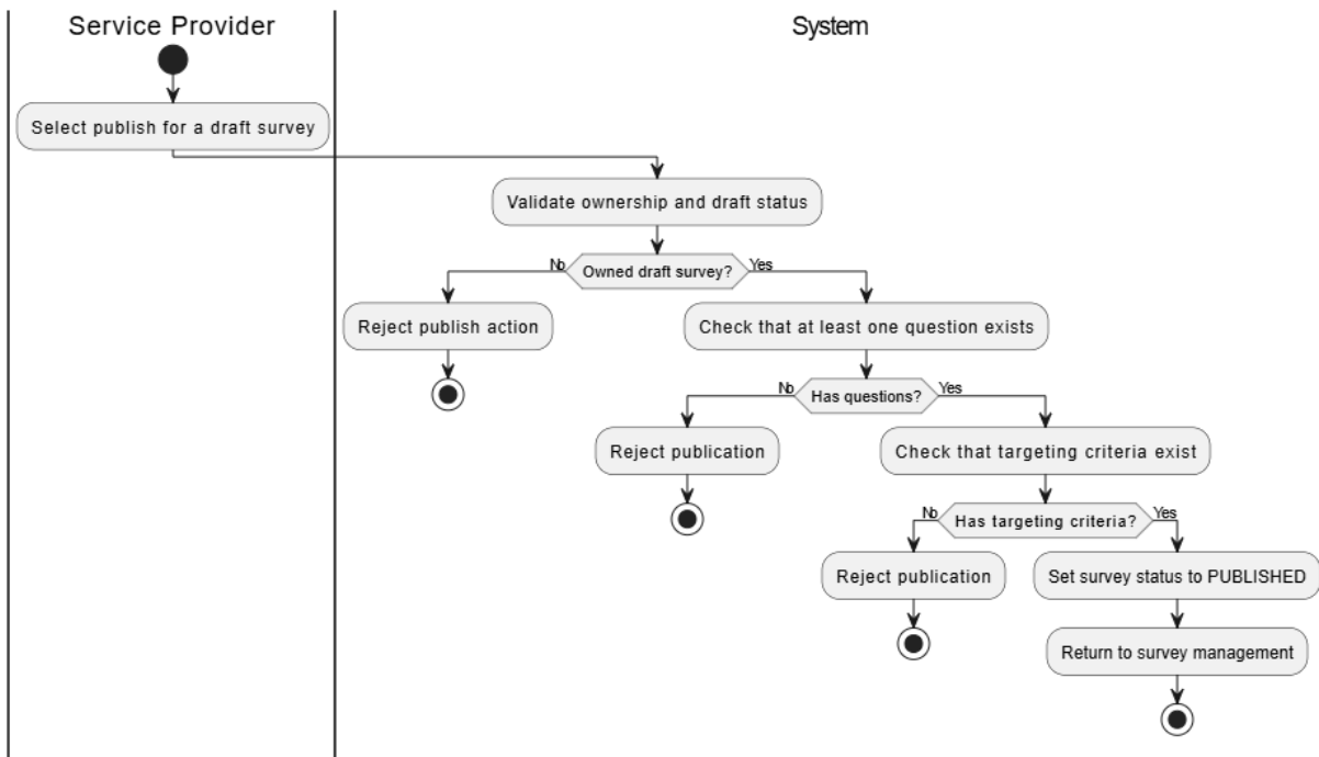
Activity Diagram - UC-11 Publish Survey
