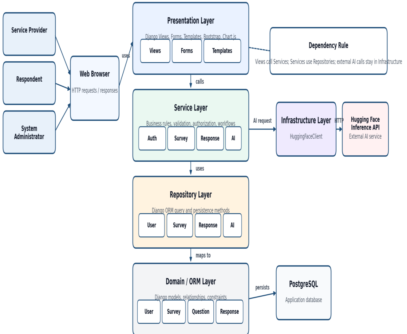
Figure B.5: System Block Diagram
