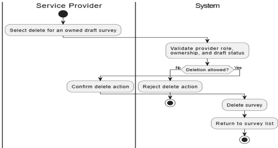
Activity Diagram - UC-07 Delete Survey
