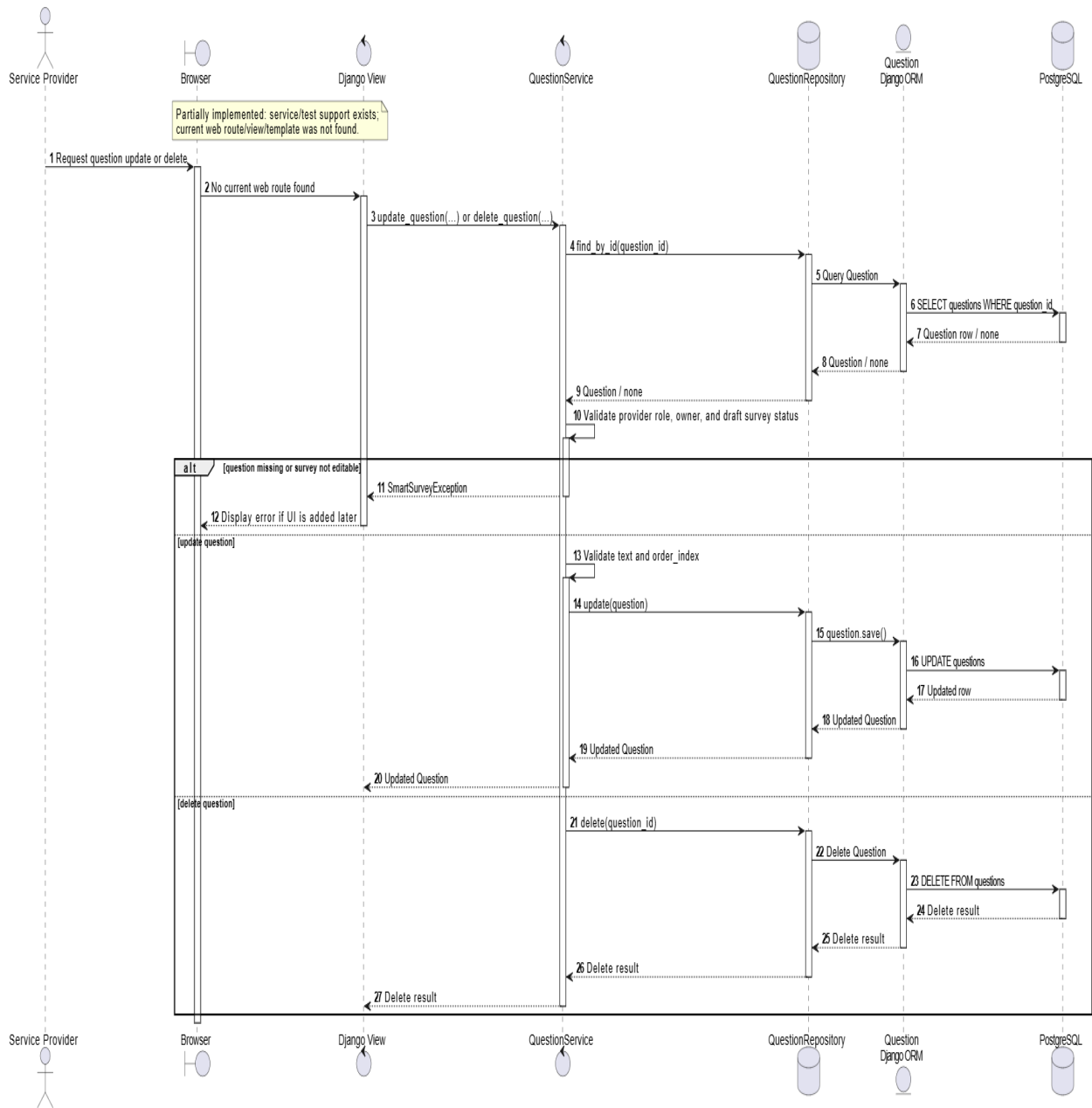
Sequence Diagram - UC-09 Edit or Delete Question
