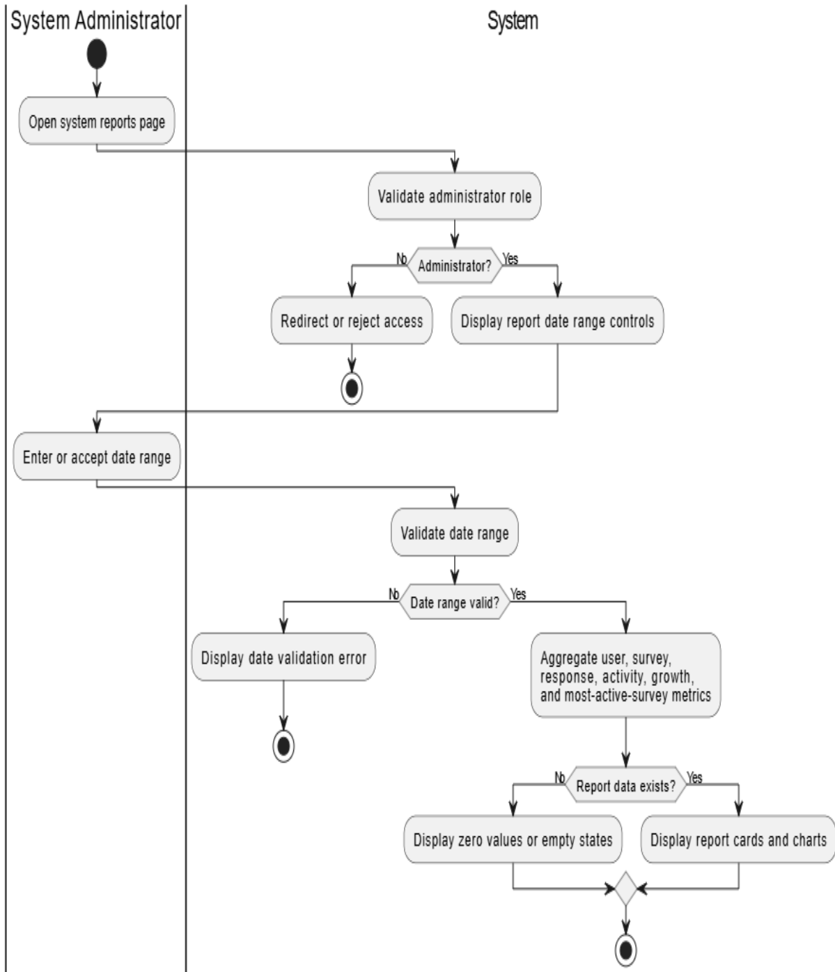
Activity Diagram - UC-19 Generate System Reports
