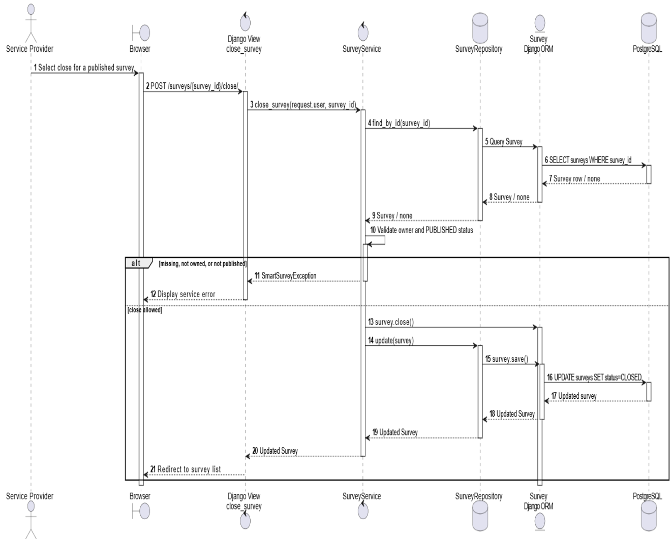
Sequence Diagram - UC-12 Close Survey
