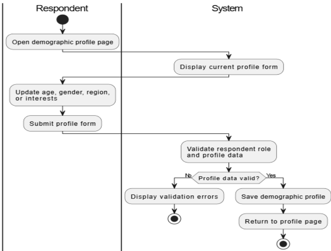
Activity Diagram - UC-14 Manage Demographic Profile
