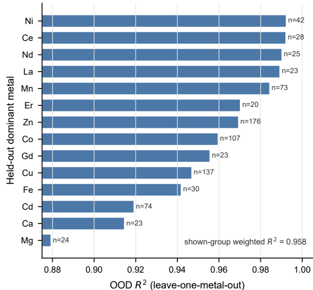
OOD by dominant metal - toluene ( n \geq 20 )
