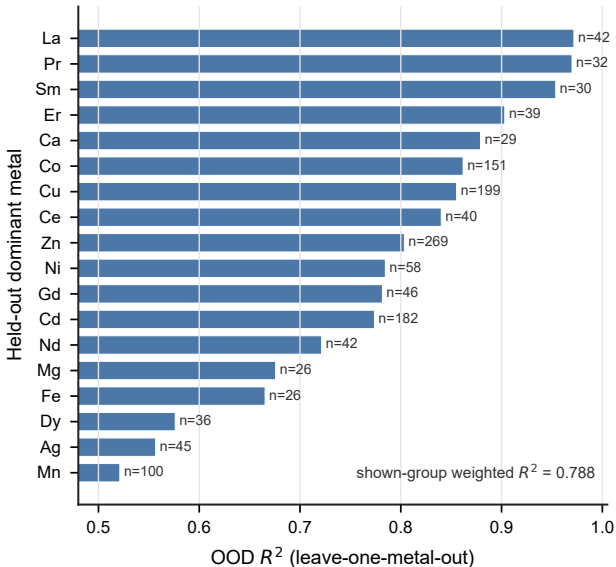
OOD by dominant metal - benzene ( n \geq 20 )
