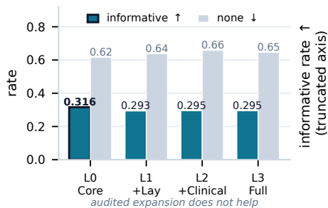
A · Vocabulary (best Top-5 each)
