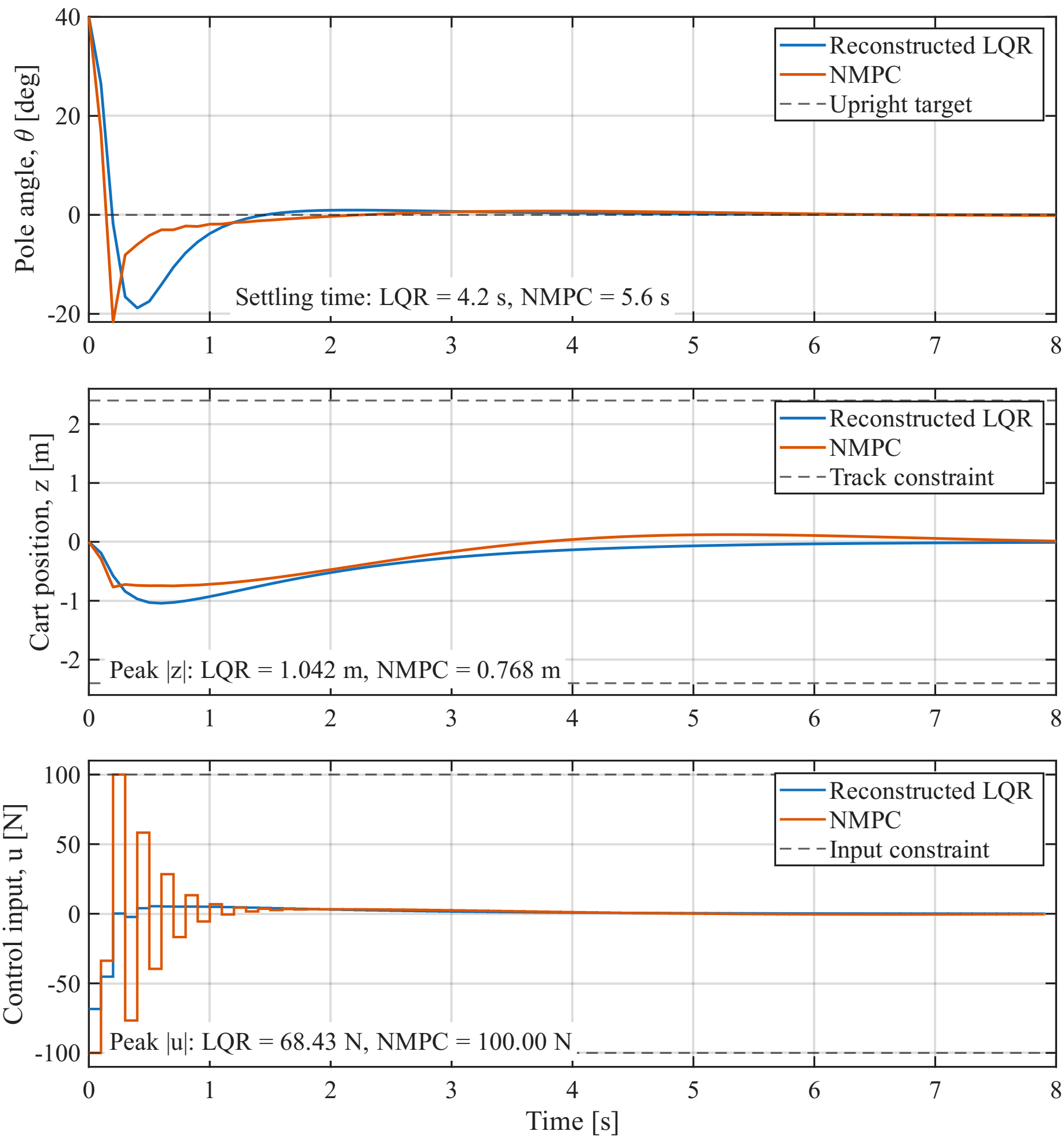
Representative 40° Challenge Cart-Pole Responses
