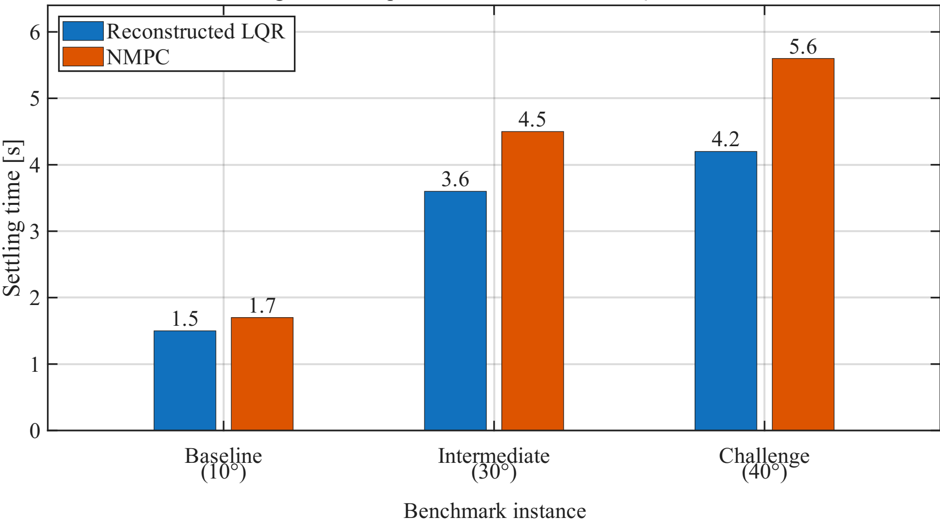
Settling-Time Comparison of Reconstructed LQR and NMPC
