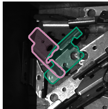
obj 13 | risk 0.977 failure | MSSD/d 0.965 — Predicted CAD silhouette
