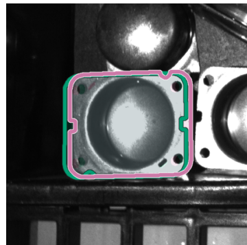
obj 5 | risk 0.001 success | MSSD/d 0.040
