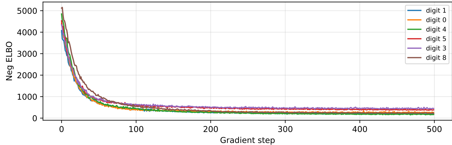
Method (c) - Loss curves
