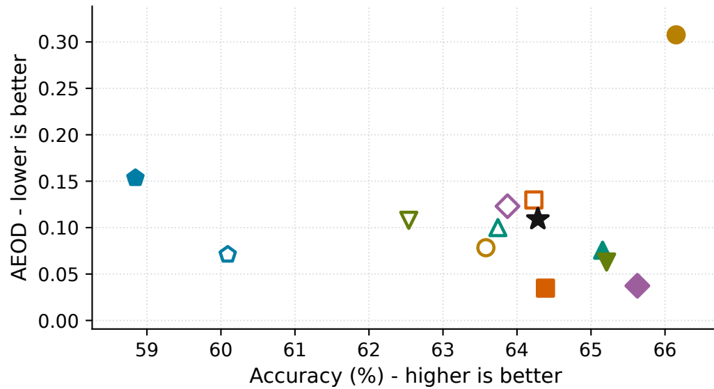
(c) COMPAS: ACC vs AEOD
