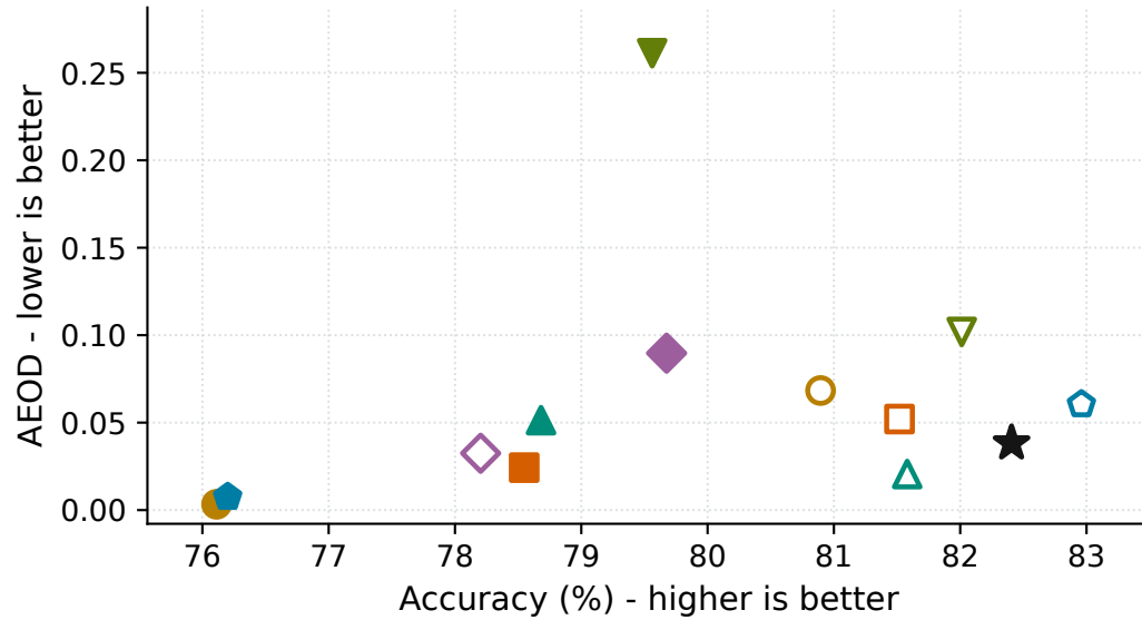
(a) Adult: ACC vs AEOD
