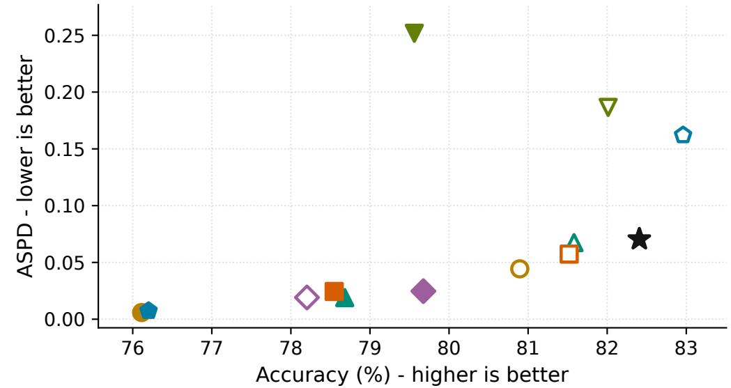
(b) Adult: ACC vs ASPD
