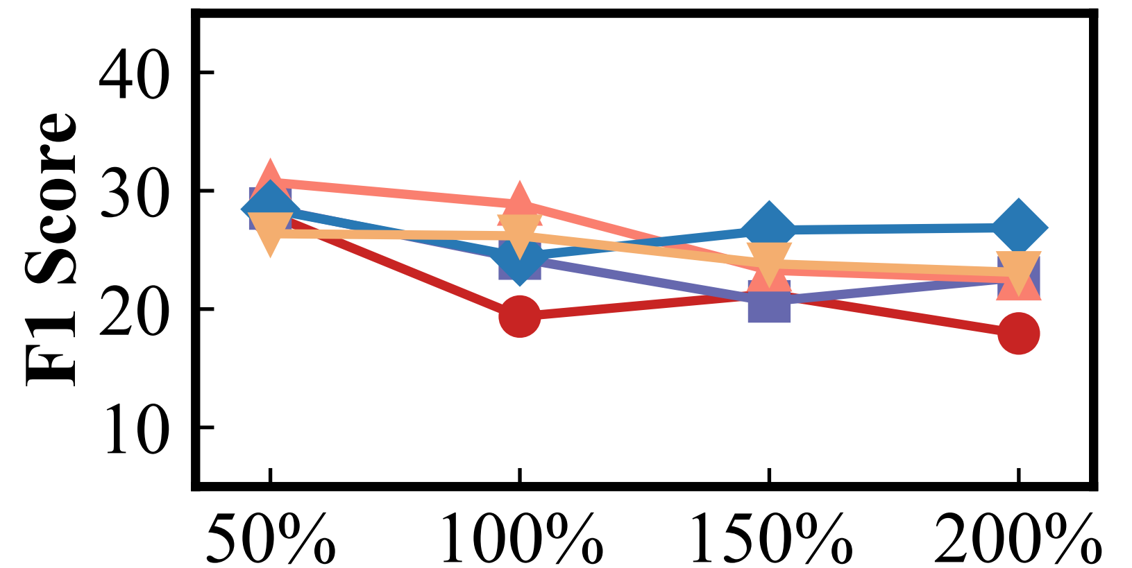
(b) Multi-Session Reasoning
