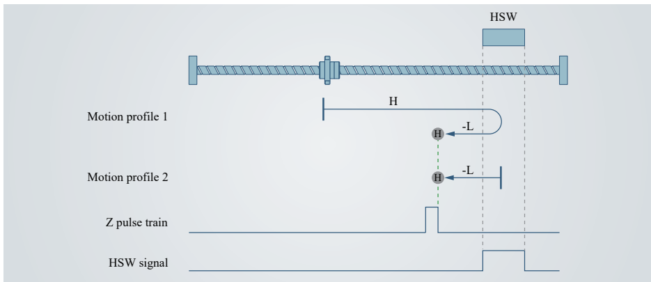
Figure 4-11 Home mode 3 profile and signal status
