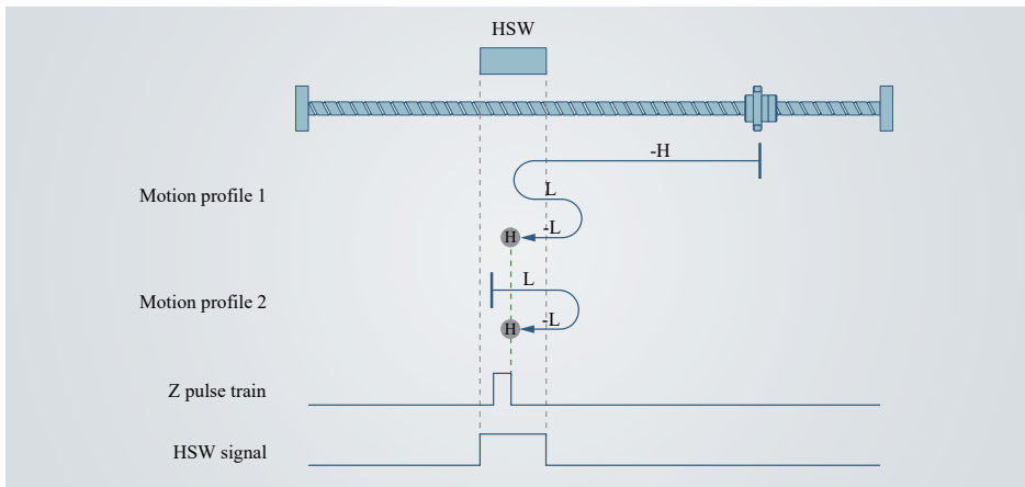
Figure 4-14 Home mode 6 profile and signal status
