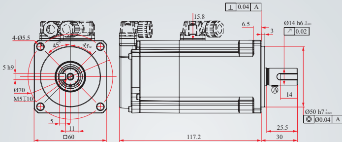
400H2B1-M17 (With brake)
