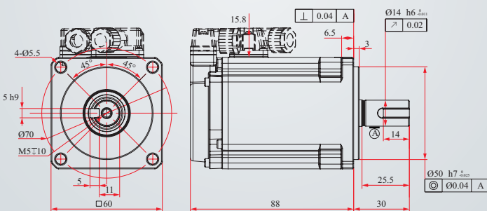
400H2A1-M17(Without brake)
