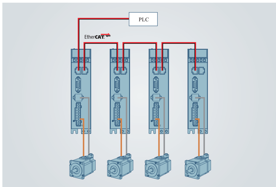
Figure 3-8 Communication networking topology
