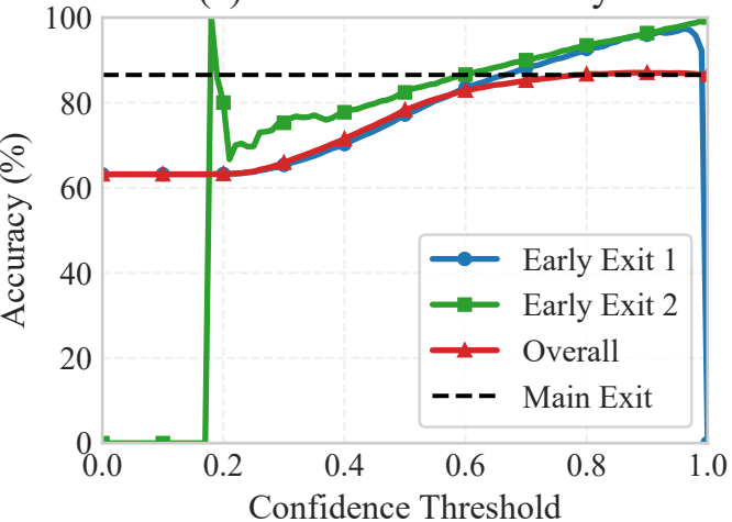
(a) Conditional Accuracy
