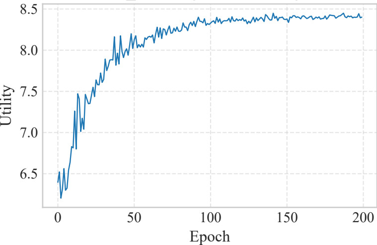
DSCI_Convergence Convergence
